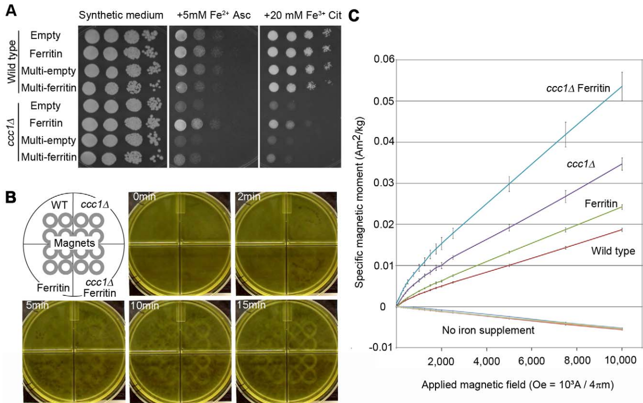
Figure 1. Magnetization of yeast. (A) Iron tolerance affected by ccc1Δ , ferritin, and \text{Fe}^{2+}/\text{Fe}^{3+} . Culture of 2.0 \text{OD}^{600} was diluted 10^2 , 10^3 , 10^4 , and 10^5 -fold in water, spotted by 10 \mu\text{l} from left to right for each strain, and grown on indicated plates. Empty, single-copy empty plasmid-harboring strain; Ferritin, single-copy ferritin gene set plasmid-harboring strain; Multi-empty, multi-copy empty plasmid-harboring strain; Multi-ferritin, multi-copy ferritin gene set plasmid-harboring strain. (B) Cell attraction towards magnet. Cell suspensions were placed over magnets ( 4 \times 4 gray circles) and a picture taken at indicated times. Corresponding video is Video S1. (C) SQUID magnetization curve. Induced specific magnetic moment was measured as a function of applied magnetic field. Lines for the four strains without ferric citrate supplementation (No iron supplement) are almost identical and overlapped; mean \pm s.d. ( n=3 ). doi:10.1371/journal.pbio.1001269.g001
