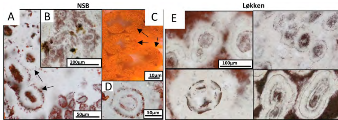
Extended Data Figure 7 | Transmitted light and reflected light images of haematite rosettes. a–d, From NSB; e, from Løkken jaspers. a, Large ( 60\ \mu\text{m} ) haematite rosettes (arrows) with cores. b, Haematite rosettes in dense haematite. c, Deformed, thicker-walled ( 25\ \mu\text{m} ) haematite rosettes (arrows). d, Concentric haematite rosette. e, Haematite rosettes from Løkken jaspers, same scale bar for all.
