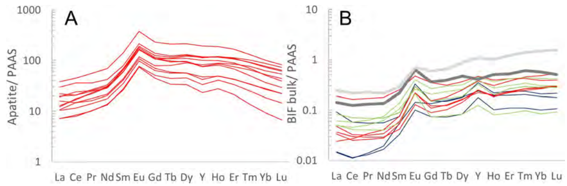
Extended Data Figure 2 | Rare earth element (REE) post-Archean Australian shale (PAAS) normalized plots. a, LA-ICP-MS REE measurements in apatite from PC0844. b, Jasper bulk rock REE measurements from PC0824 (dark grey) and PC0844 (light grey). NSB (red 15 and green 16 ) and Isua 51 (blue) iron formation bulk rock REE.
