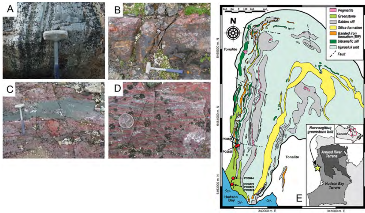
Extended Data Figure 1 | Field photographs of the NSB iron formation outcrops. a, Bands of magnetite and chert. b, Jasper (top red layer) in contact with Fe-rich carbonate (bottom grey layer). c, Layered jaspers with meta-volcanic layers. d, Layered jasper; predominantly bands of grey haematite and haematitic chert. e, Field location, local geology and sample locations (red spots).
