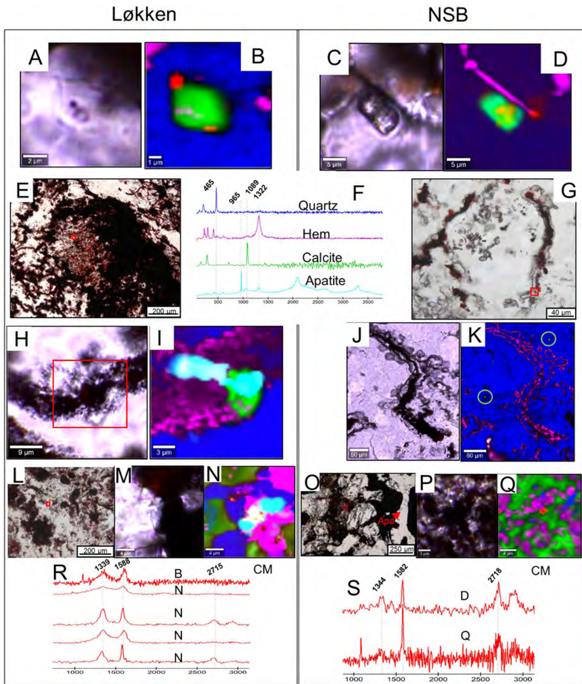
Extended Data Figure 5 | Carbonate–apatite and carbonaceous material in the NSB and Løkken jaspers in association with haematite filaments.
