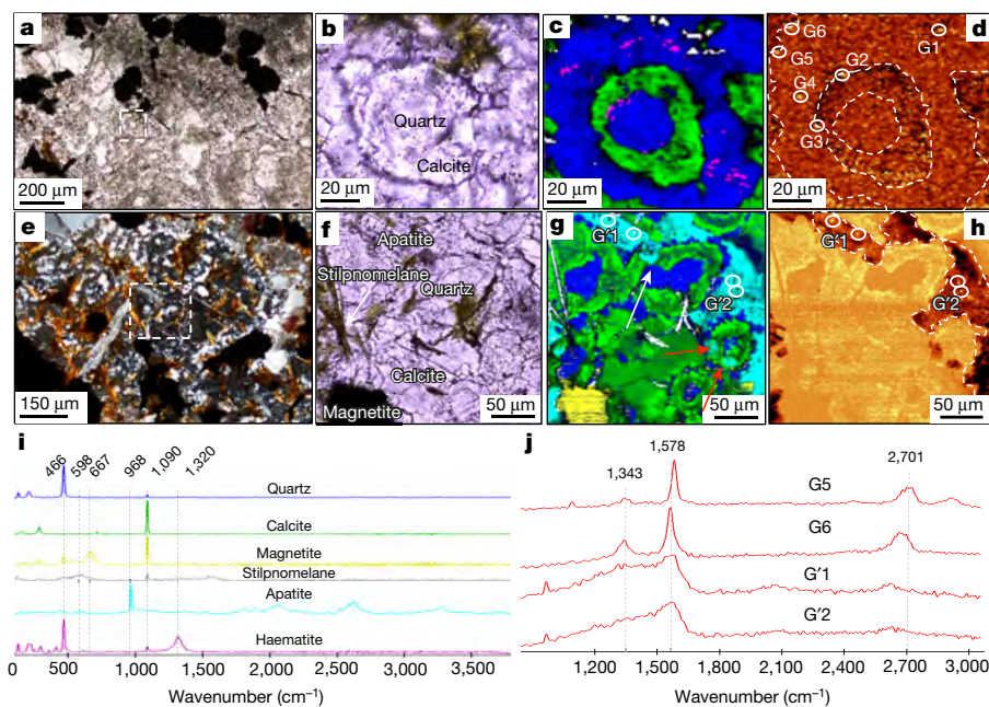
Figure 3 | Carbonate rosettes from the NSB.
