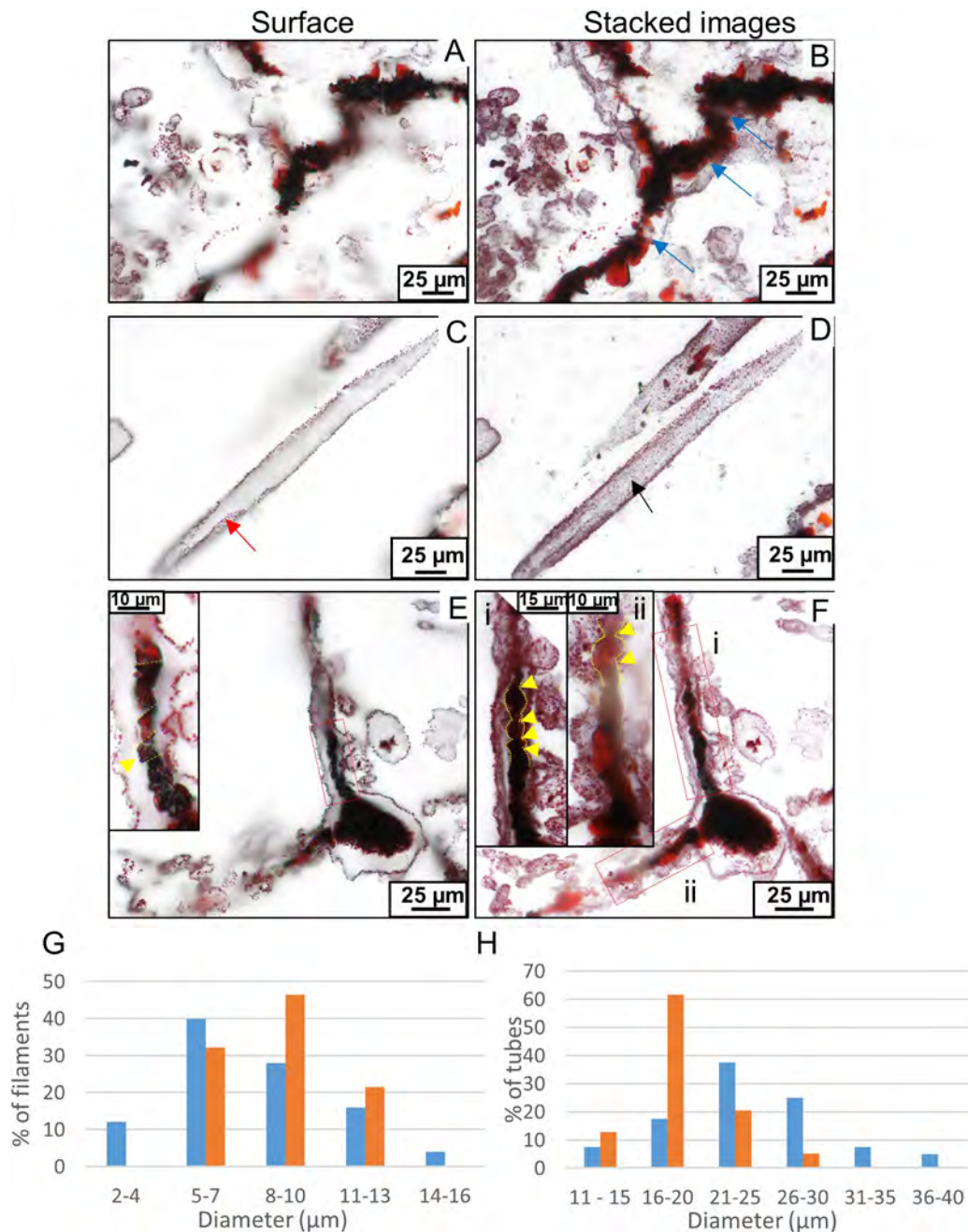
Extended Data Figure 4 | Photomicrographs taken in plane-polarized light with reflected light of haematite tubes and filaments. Images in left column are taken at the surface of the thin section. Images in right column show a series of stacked images using the Z-project function in ImageJ. Stacked images are formed of 8–9 sequential images taken at 2- \mu\text{m} intervals through the thin section. a , Branching haematite filament. b , Stacked image of a . Arrows point to loose coils. c , d , Hollow tube truncated partially at the surface showing both the top ( c , red arrow) and bottom surface ( d , black arrow) of the tube. e , Twisted haematite filaments emanating from haematite knob at varying angles and depths through the
