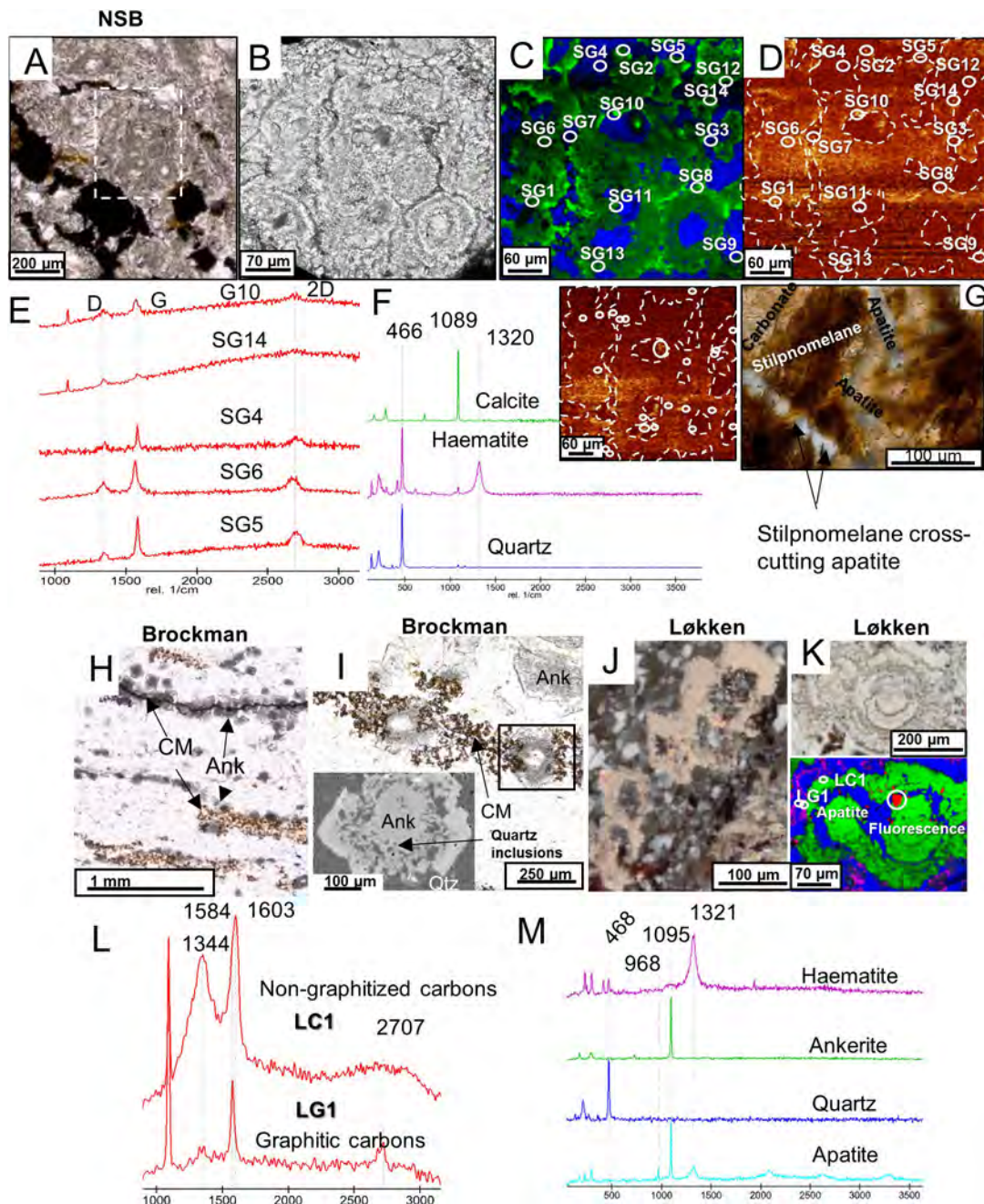
Extended Data Figure 6 | Carbonate rosettes. a , Transmitted light image of calcite rosettes from the NSB. b , c , Transmitted light and Raman images of target area (dashed outline from a ). d , Graphite Raman filter map (filter: 1,580 \text{cm}^{-1} , width 40 \text{cm}^{-1} ). Circled pixels are graphite grains. e , Raman spectra of selected graphite particles. f , Average Raman spectra for Raman map in c with inset of haematite Raman filter map (filter: 1,320 \text{cm}^{-1} , width 30 \text{cm}^{-1} ). Circled pixels are haematite grains. g , Stilpnomelane laths overgrowing apatite in the NSB. h , Ankerite rhombohedra envelop
