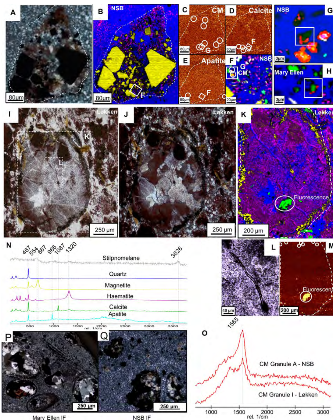
Extended Data Figure 9 | Granules from the NSB and from the Løkken jaspers. a , Transmitted light image of a granule in the NSB. b , Raman map of the granule in a . c , Carbonaceous material Raman filter map (filter: 1,580\text{ cm}^{-1} , width 80\text{ cm}^{-1} ). d , Calcite Raman filter map (filter: 1,089\text{ cm}^{-1} , width 20\text{ cm}^{-1} ). e , Apatite Raman filter map (filter: 965\text{ cm}^{-1} , width 30\text{ cm}^{-1} ). f , One micrometre spatial resolution Raman scan of part of the granule in a . g , Raman scan ( 360\text{ nm} resolution) of boxed area in f (yellow and white colours are colour combination artefacts). h , Raman scan ( 500\text{ nm} resolution) of a portion of the interior of the Mary Ellen granule in Fig. 4b, showing carbonaceous material coating a carbonate grain, like carbonaceous material coating a carbonate grain in the NSB granule in a . i , Transmitted light image of granule from the Løkken jasper.
