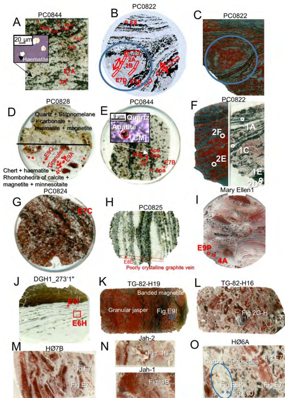
Extended Data Figure 3 | Thin sections of samples in this study (see Supplementary Information for localities). Inset in a shows reflected light image of small, sub-spherical chalcopyrites with haematite. Red outlines mark haematite tubes and tube-like structures. Red arrows show the orientation of tubes. Blue circles highlight concretion structure
