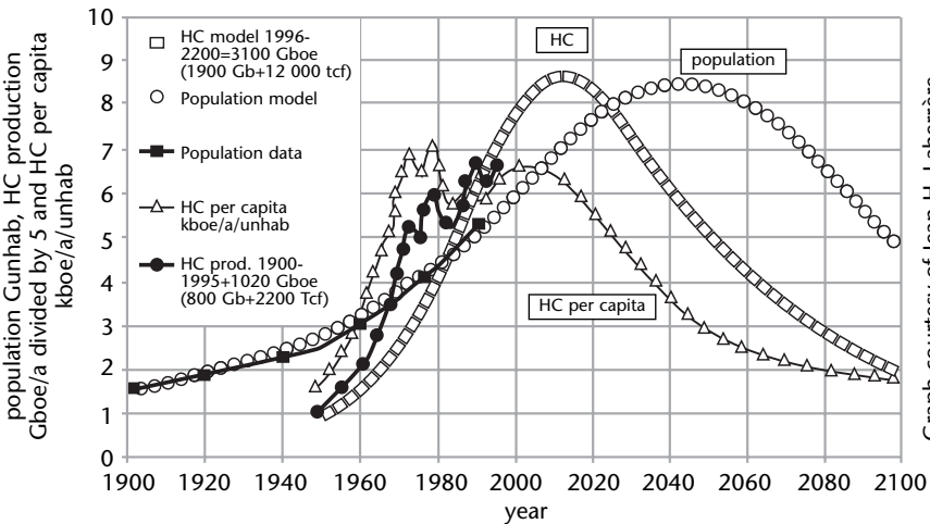
Scenario of world's population and hydrocarbons (liquids + gas) production: 1900-2100
