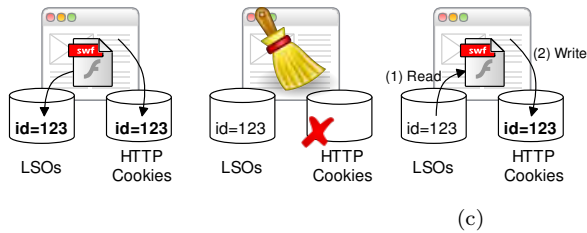
Figure 2: Respawning HTTP cookies by Flash evercookies: (a) a webpage stores an HTTP and a Flash cookie (LSO), (b) a user removes the HTTP cookie, (c) the webpage respawns the HTTP cookie by copying the value from the Flash cookie.
