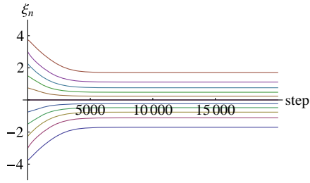
FIG. 3. Convergence of the ensemble of world-particles x_n = (x_1, \dots, x_N) for N = 11 towards the ground-state configuration as a function of the step number in the iteration algorithm described in the text. Here, dimensionless positions are used, \xi_n = \sqrt{2m\omega/\hbar}x_n , as per Eq. (41), and the temporal step size is \Delta t = 5 \times 10^{-2}\omega^{-1} . As the plot shows, convergence is complete by step number 6000, at which the distribution of worlds is close to the Gaussian quantum ground state.
