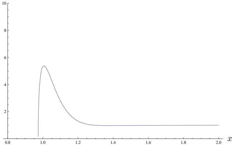
Figure 1: The function \sqrt{F_1(x)} with F_1(x) = 1 - 1/x^7 + 0.000001f_1(x) .
