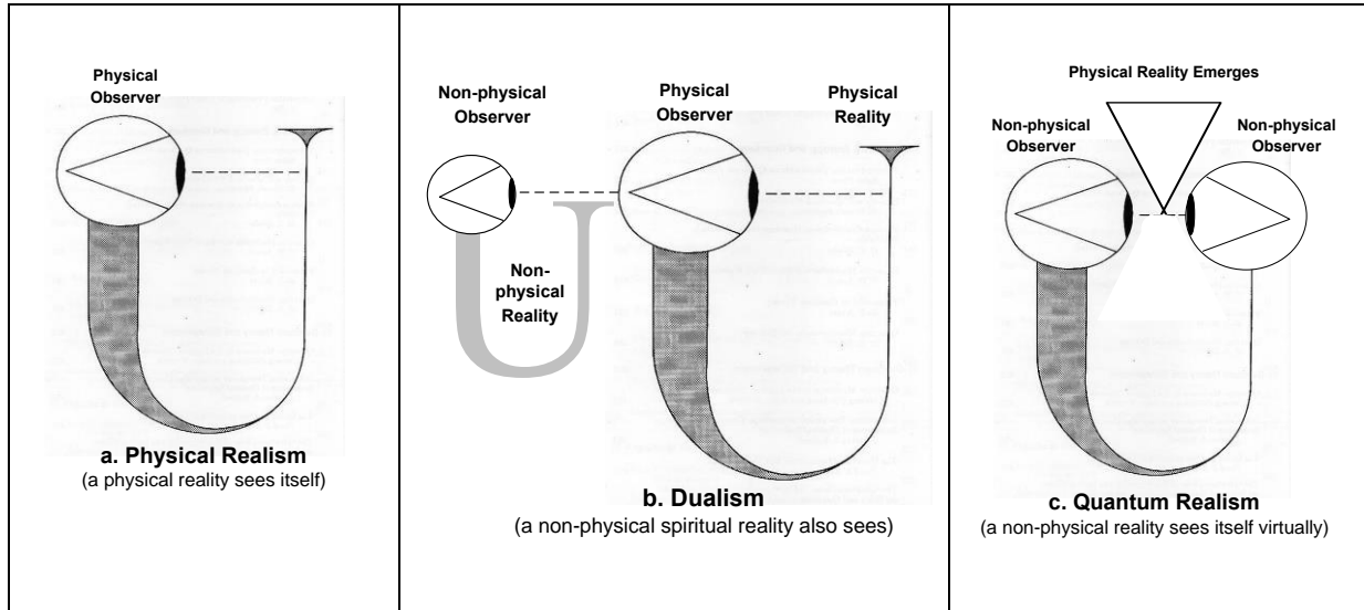
Figure 1.2. The “What is Reality?” candidates
