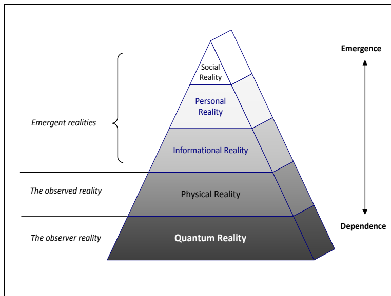
Figure 1.6. Physical reality emerges from quantum reality
