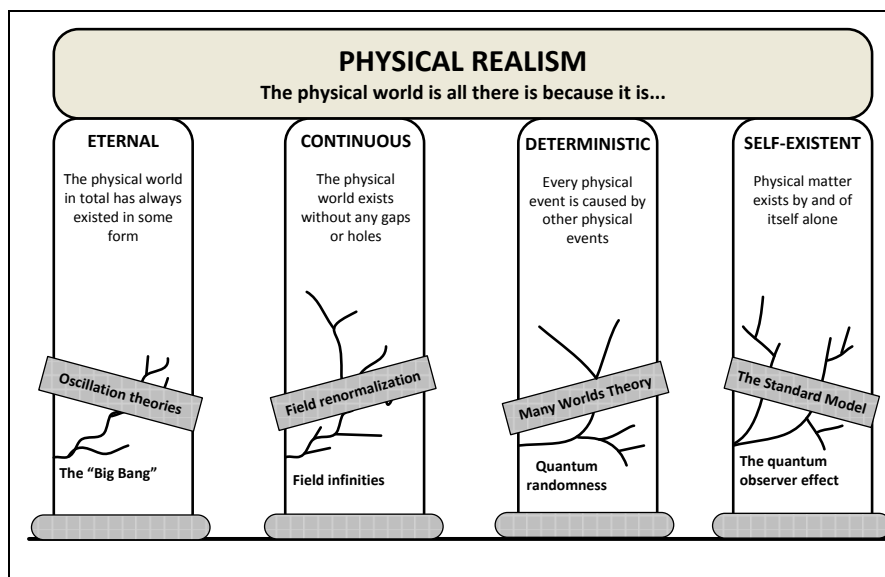
Figure 1.7 The four pillars of physical realism
