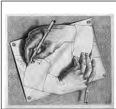
Figure 1.3. The physical universe can't do this 14
