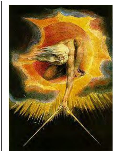
Figure 1.1 The Ancient of Days measures the universe 2
