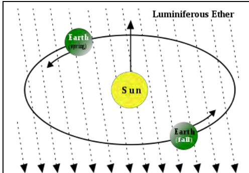
Figure 1.4. A physical ether 16
