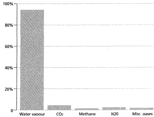
Figure 5: This graph of greenhouse gases puts the hysteria about carbon dioxide into perspective. If you want to stop the greenhouse effect then ban clouds and condensation and, by the way, without a greenhouse effect and carbon dioxide (CO 2 ) there would be no human life.
