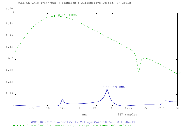
6. Voltage Gains
