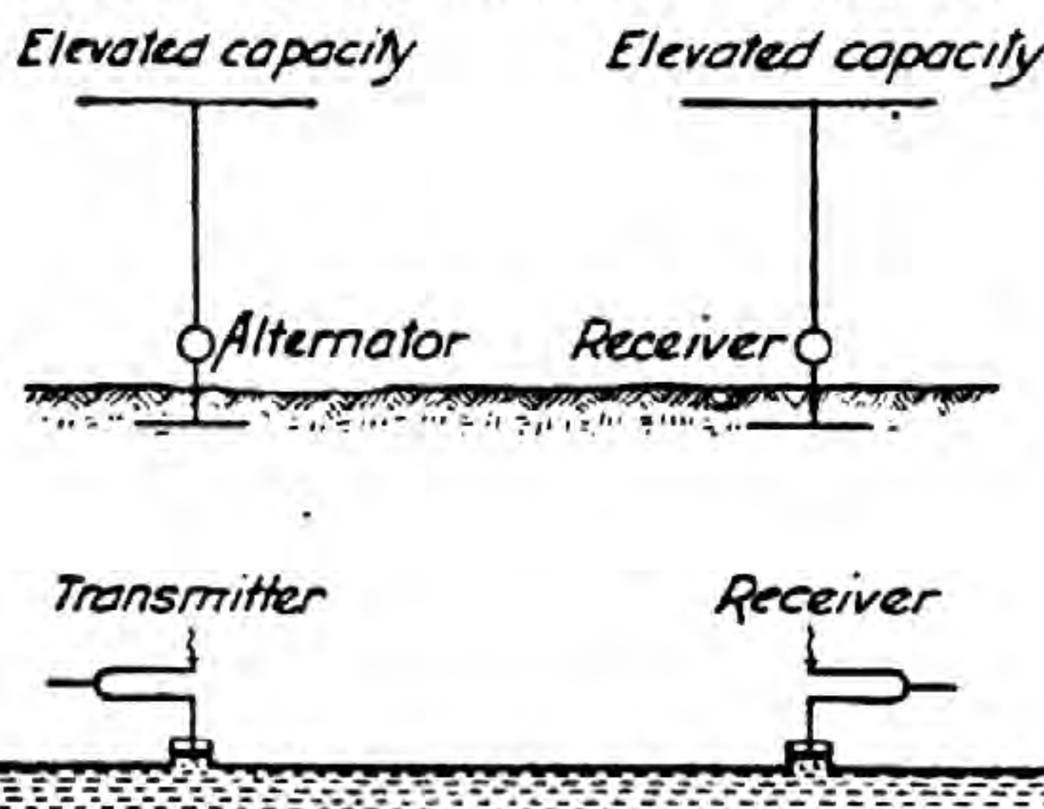
Transmission of Electrical Energy Thru the Earth as Illustrated in Tesla's Lectures Before the Franklin Institute and Electric Light Association in February and March, 1893, and Mechanical Analog of the Same. Fig. 7.
