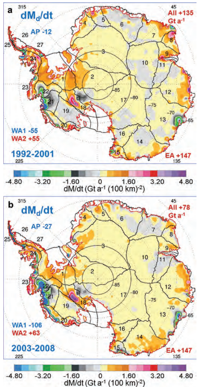
Fig. 11. Maps of the dynamic-driven mass changes, dM_d/dt , (a) for 1992–2001 ( dH/dt from ICESat used south of 81.5^\circ \text{ E} ) and (b) for 2003–08. In WA1, the net dynamic-loss rate increased from 55 \text{ Gt a}^{-1} to 106 \text{ Gt a}^{-1} . Dynamic thickening (excess of long-term accumulation over ice flux) occurred over WA2 and EA in both periods. Dynamic thickening ( 27 \text{ Gt a}^{-1} in 2003–08) is strongest in DS18 in an area inland from Kamb Ice Stream that stagnated 150 years ago. Similarly, the dynamic thinning in Eastern DS17 and Western DS18 is inland of Mercer and Whillans Ice Streams, which restarted flowing 400 years ago.
