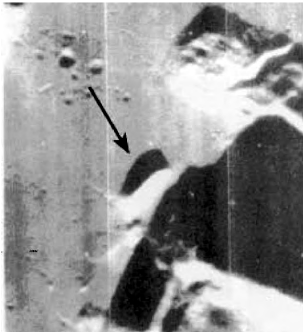
Fig. 69. Figure on the left - Figure 64 a. NASA LO IV, Ah: 187 2 . It shows a large cloud zigarrenformige or object.
