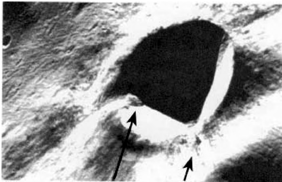
Fig. 128. Hasselblad Photo Ne 15-13181 (enlargement). A kind of machine seems to blow the earth from the crater, which looks suspiciously like mine. Also note the two oval objects south of the crater rim.
