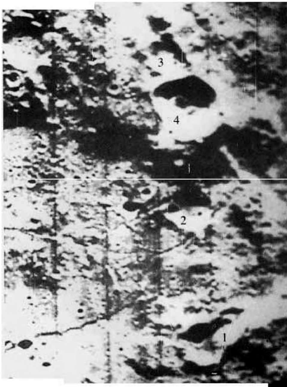
Fig. 75. Photo by NASA LO II No.: 161'; magnification image of the eastern part of 67th Note: No. 1 - the large construction, nr 2 and nr 3 - two platforms, No. 4 - maybe another platform?
