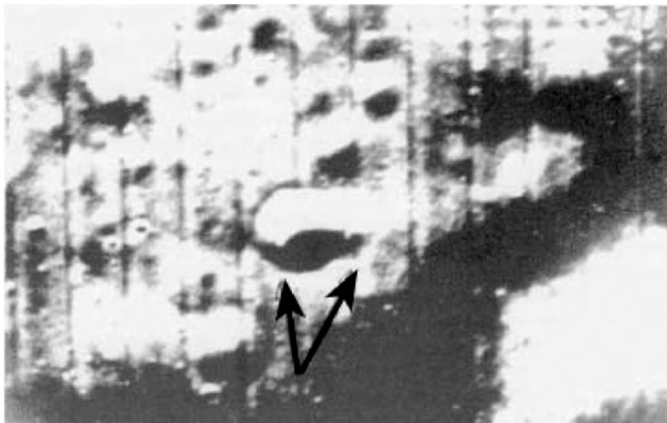
Fig. 46. Lunar Orbiter III (enlargement) of a crater, the two Crater walls in this show, which is located in the southeast of Mare Tranquillitatis
