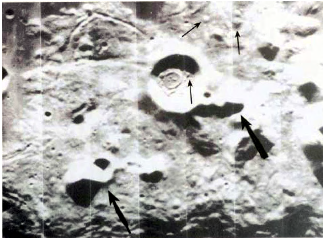
Fig. 70. Right figure - Figure 64: NASA LO 1I7, Ne Photo 1872 (Enlargement), area of the Alpine valley on the moon. Look for the large oval Object (UFO or cloud) 1.6 Kilometers above the large Crater. In addition, still more clouds on the top left To see photo and three domes, two to the left of the crater and top left of the crater
