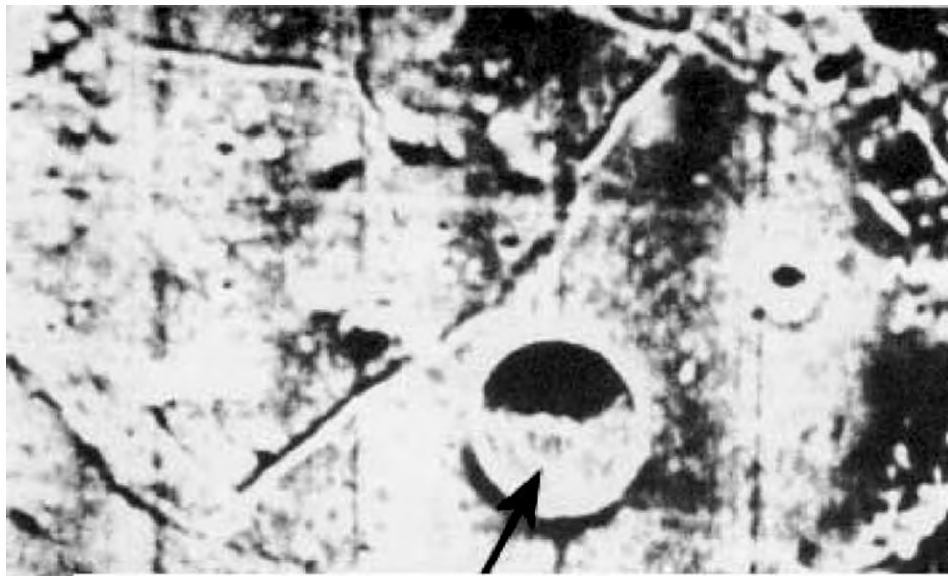
Fig. 76. Photo by NASA LO IV, N. 86 3 , and the crater Posidonius. Note the two oval objects on the bottom of the crater and clouds in the north-west, covering the great gorge.
