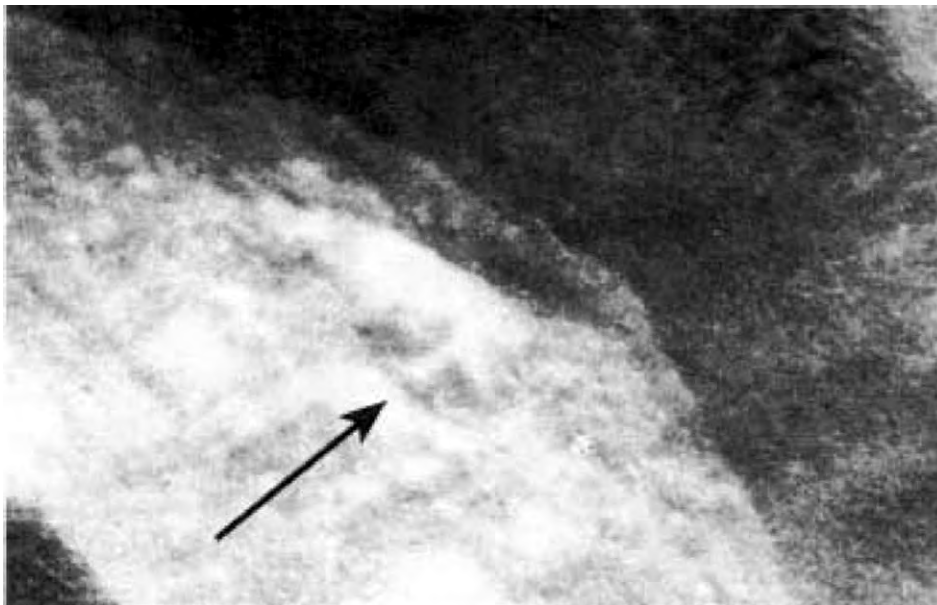
Fig. 130. Photo of Apollo 8, Ne 8-17-2704 (enlargement). This photo shows two pyramidal structures on the moon.
