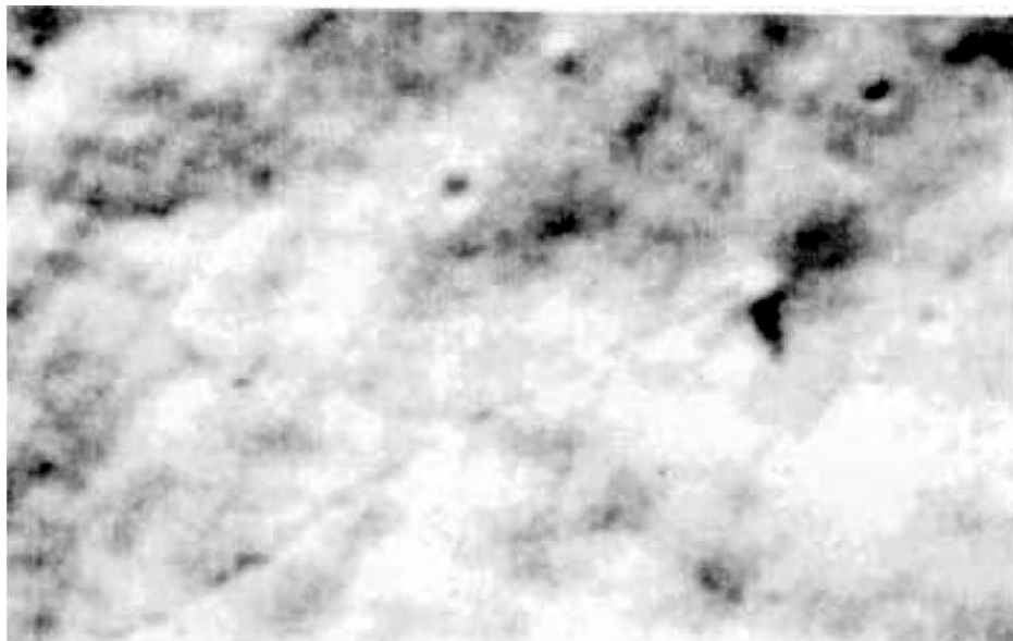
Fig. 26. Figure 25: LO V NASA photo, no 67-1-1-1135 (enlargement). The small object, 4.6 meters in diameter, rolled about 370 meters up the hill and down
