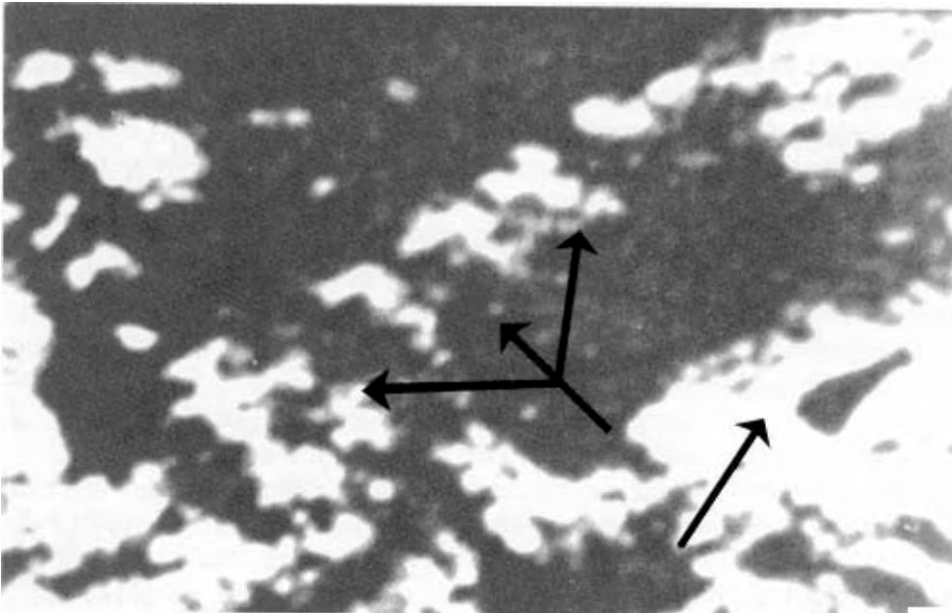
Fig. 6. Figure 7: In the mountain peaks cut platforms that extend over 48 kilometers. South of Archimedes. Each platform seems to be a letter or symbol to represent. Note also the large structure in the valley below.
