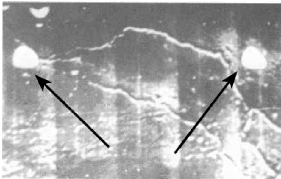
Fig. 59. (enlargement): LO-IV-Photo of ponds or lakes, which reflect sunlight. Also note that it seems as may be water in these river beds.
