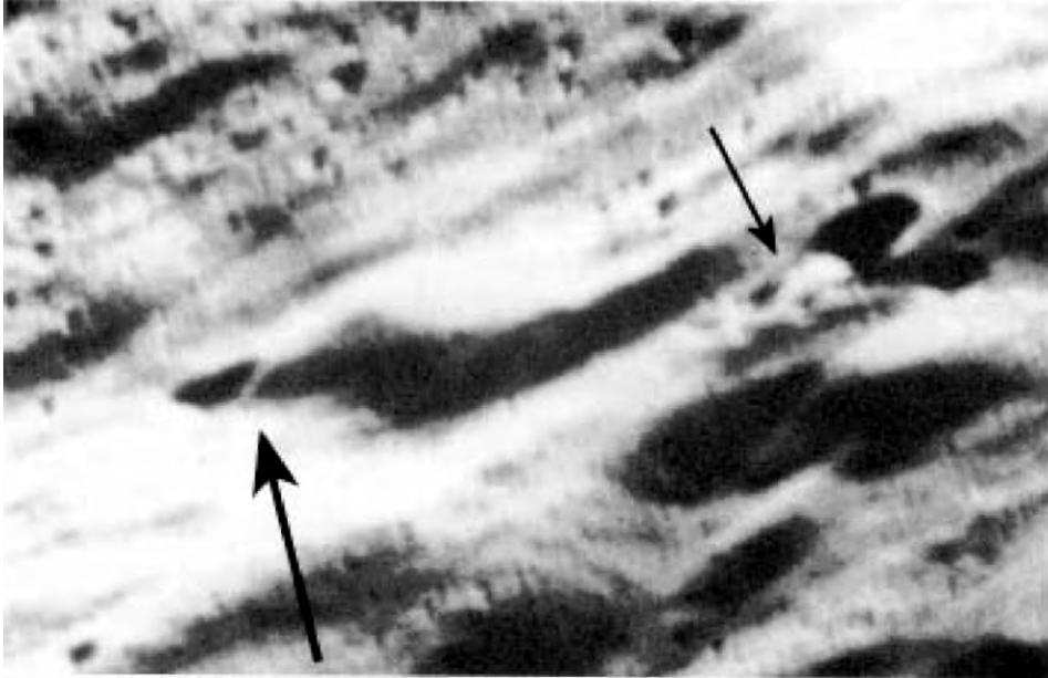
Fig. 79. Photo by NASA Apollo 16-19273 (enlargement), northeast of the crater King. Note the dust being blown up left out of the crater. Anyone operating on the moon mining?
