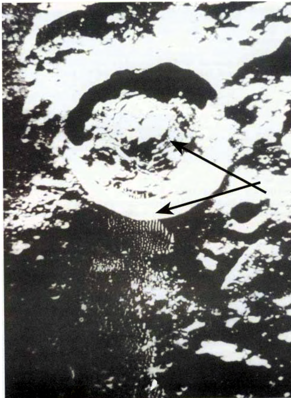
Fig. 49. Figure 44: NASA's Lunar Orbiter Ne MR 168 (enlarged). The crater Vitello. Note the fluffy clouds below Vitello. Watch out for the Platform in the center of the crater.
