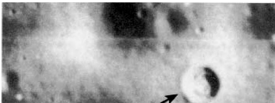
Fig. 108. Lunar Orbiter III, No. 194 Photo 3 (enlargement). Note the large letters .. S "in the interior of the crater in this photo.
