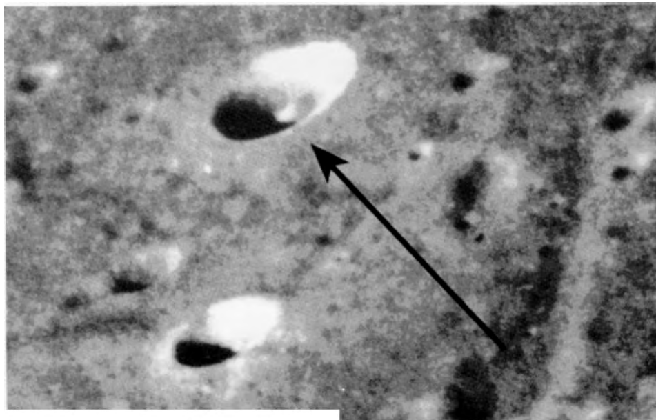
Fig. 34. Apollo 14, Picture No. 14-10116 (enlargement). The photo shows a white dome in the crater.
