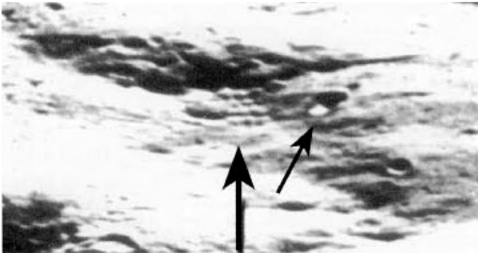
Fig. 80. Photo by NASA Apollo 16, No. 16-19265 (enlargement). Note the ten objects in addition to a specially cut crater, which looks much like an underground hangar, parked neatly in rows.
