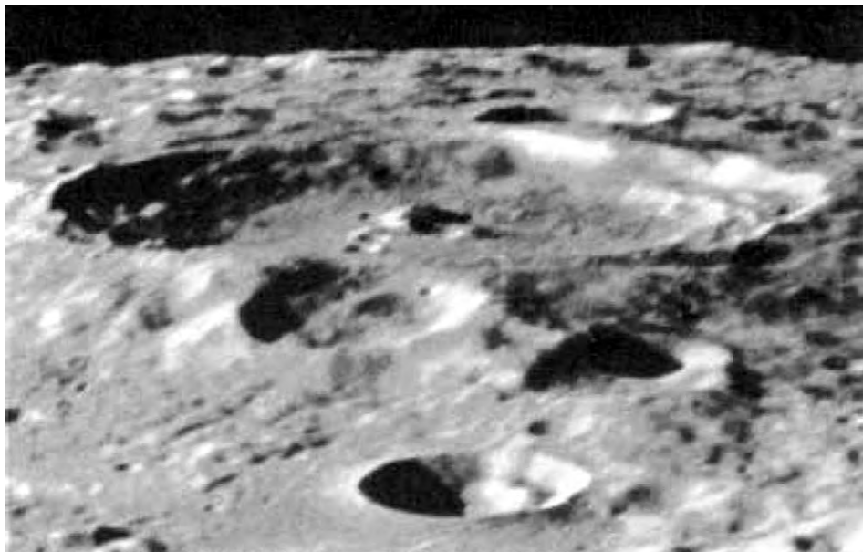
Fig. 138. Figure 132: Allollo 13 - near the crater Bullialdus. Note another Area in which there are apparently more activity, smoke, dust or mud flows from the smaller to the larger craters including crater above
