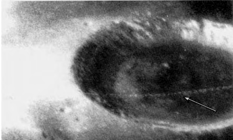
Fig. 25. Apollo 16 Photo No.: 16-19067 (enlargement) Photo by NASA. About forty-eight km impression straight tracks running up and down the hill and leave marks that are identical to those in figure 23. Moon back.
