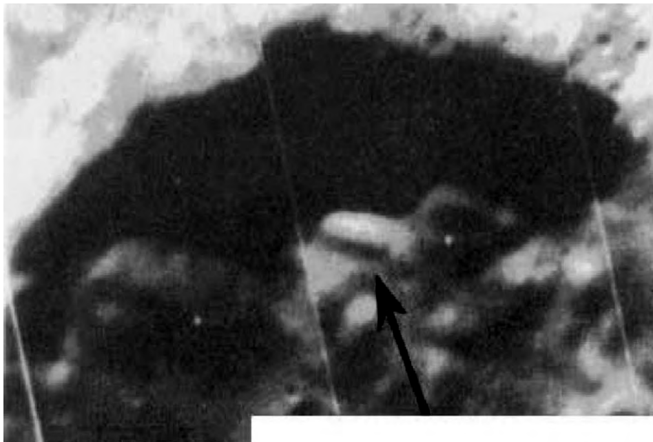
Fig. 97. Figure 91: Photo of Lunar Orbiter IV NASA's No. LO IV 89 '. White cigar-shaped Object in the vicinity of the crater Romer
