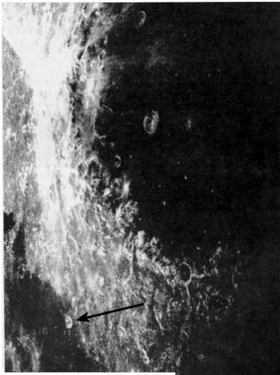
Fig. 82. Photo by NASA Apollo 16, No.: AS-16-121-19438th Note the large icon on the inner wall of the crater left near the Sea of Tranquility.
