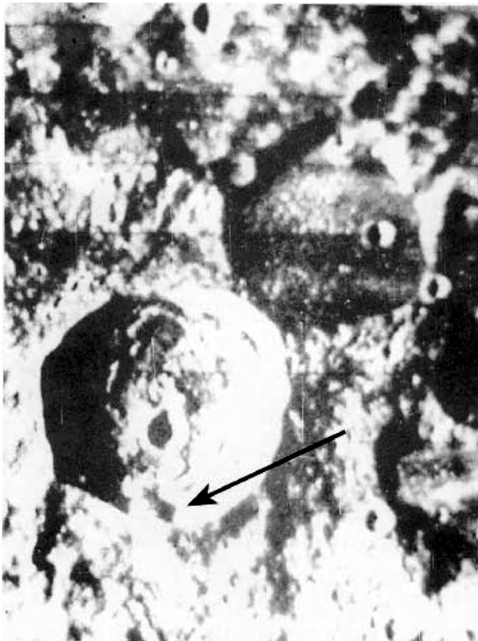
Fig. 62. Photo of Luna NASA - Orbiter IV, Ni, HR 161 3 (enlargement), the crater Prosper Henry: Please note the large white cloud that hangs over the lower wall of Prosper Henry. Top right corner of the crater next to Prosper Henry are still visible more clouds. Pay attention also to the various objects near the oval cloud in the middle crater
