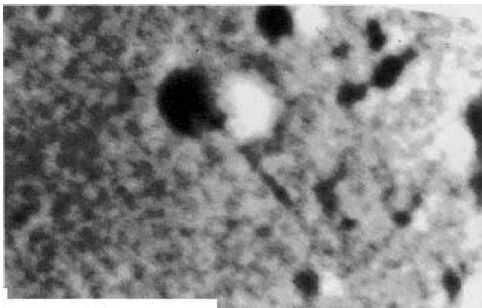
Fig. 120. Photo of Apollo 15 (enlargement). A long tube that rises from a crater.
