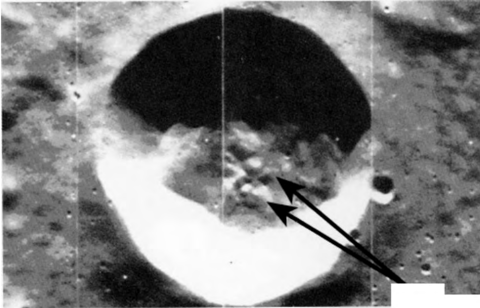
Fig. 30. NASA's Lunar Orbiter photo IV, No. 168-H3, moon back (enlargement). Two domes on the crater floor g3
