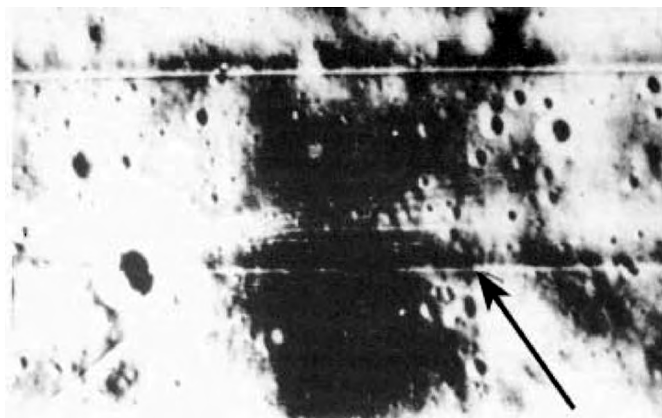
Fig. 47. Photo of Lunar Orbiter III (enlargement) of the same area as on picture 42nd The traces are clearly visible.
