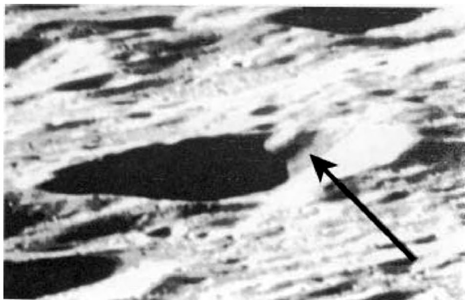
Fig. 104. Photo of Apollo 16, No. 16-18918 (enlargement). Oval object in the large crater
