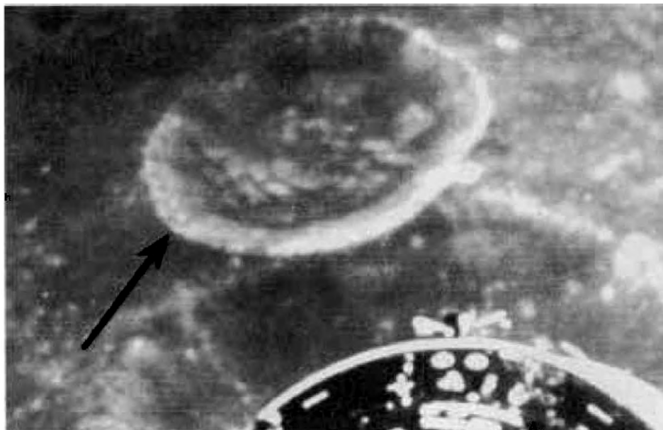
Fig. 105. Photo of Apollo 10, Ne unknown. Four white egg-shaped objects that are parked in the large crater.
