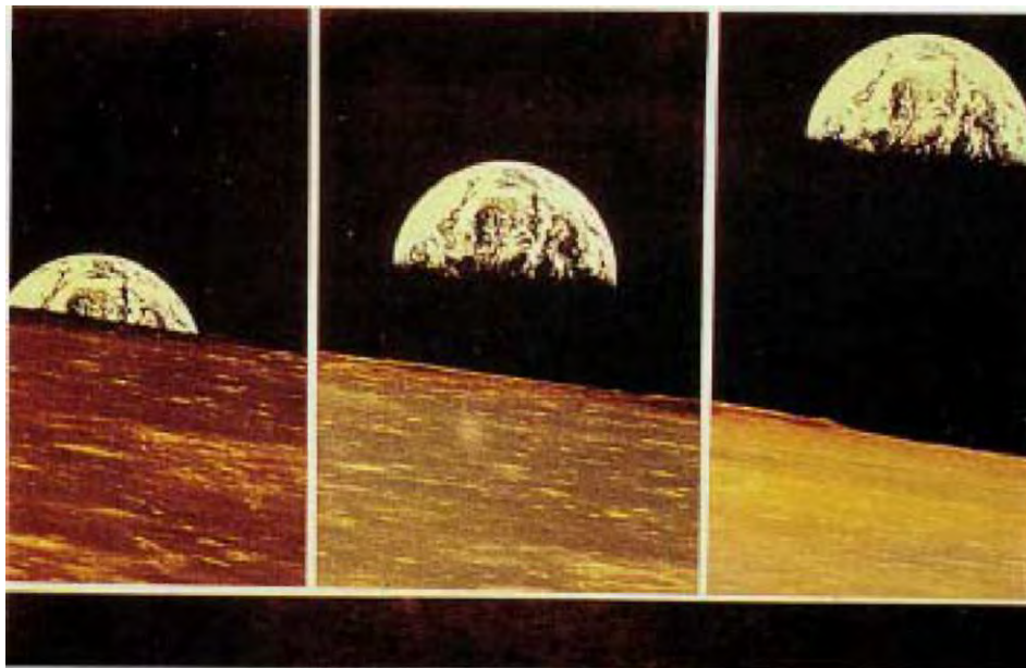
Fig. 37. The Seen "rising" of the earth from the moon.
