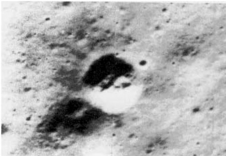
Fig. 107. Figure 101: Photograph by LO III, No. 200 3 (enlargement). Strange objects in the This crater is parked.
