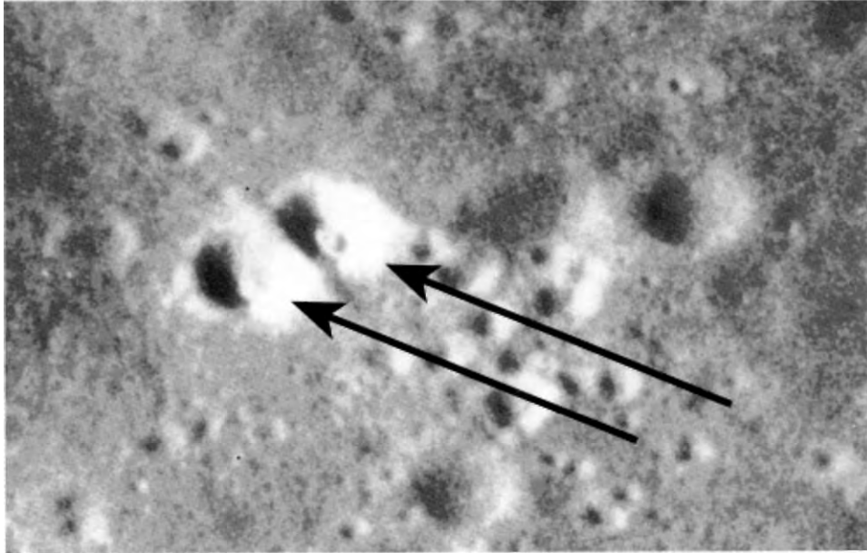
Fig. 33. Apollo Hasselblad Photo No. 16-19081 (enlargement). A double crater with two dome-like structures or objects. Note the long object between the craters.
