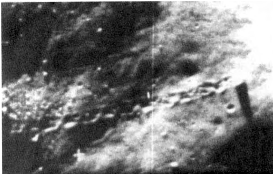
Fig. 24. LO V NASA photo, no 67-1-1-1135 (enlargement). The small object, 4.6 meters in diameter, rolled about 370 meters up the hill and down
