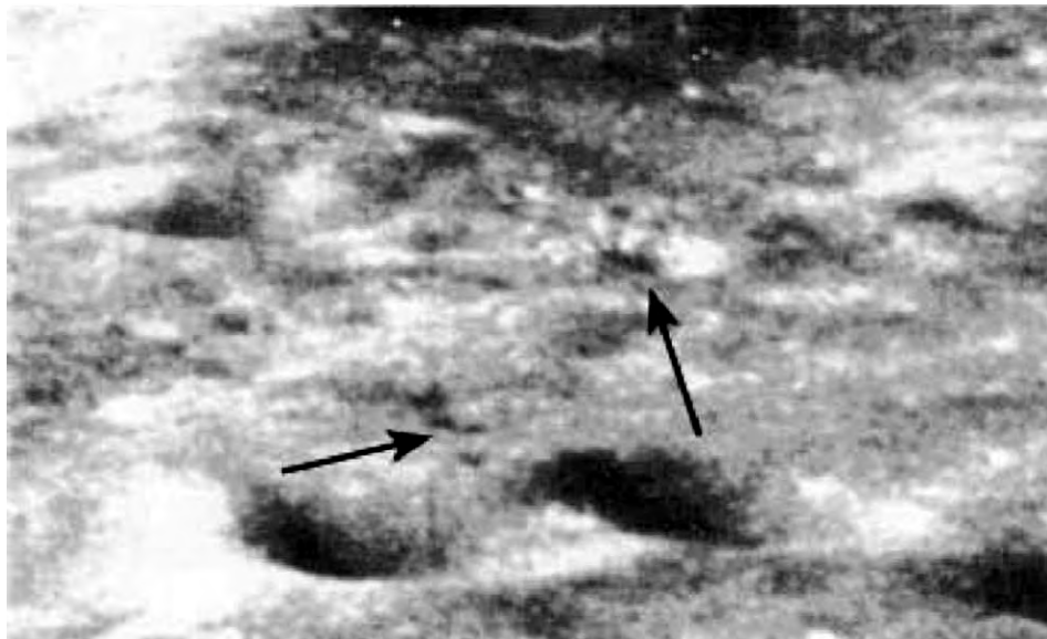
Fig. 121. Photo of Apollo 16, No. 16-19376 (enlargement). Another tube or pipe between two craters. Also note the strange objects in the smaller crater about
