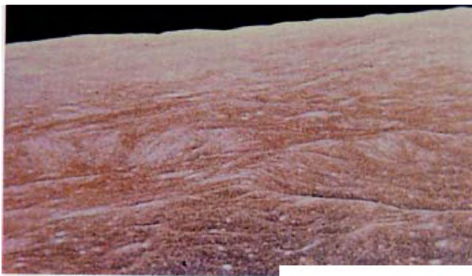
Fig. 44. Color photo of Apollo 8 from the side of the moon. The moon on the original color appears in full autumn colors. Note the clearing in three rows near the edge of the largest crater on the right.
