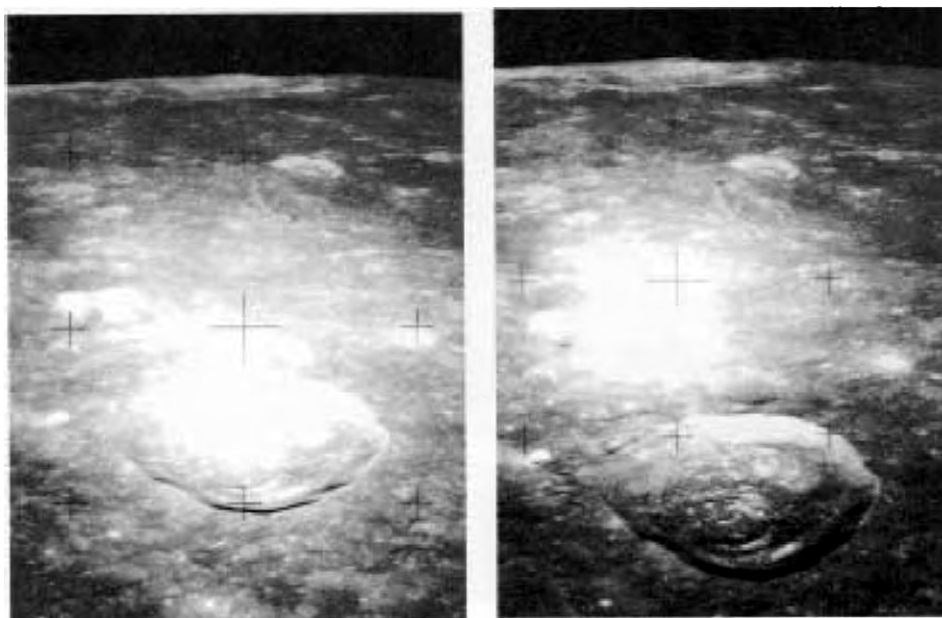
Fig. 68. Photos 62 and 63: Photos from Apollo 14, No. 14-10279 and 14-10280. Note that the large cloud or haze has moved north of the crater, covered them / it.
