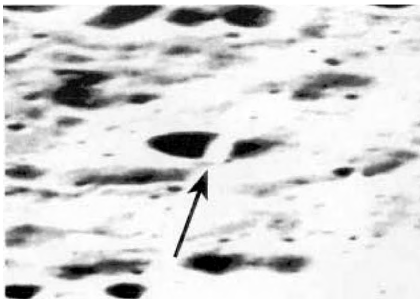
Fig. 116. Apollo 16, Ni: 16-18923 (enlargement), this photo of Apollo 16 shows a crater that appears designed.
