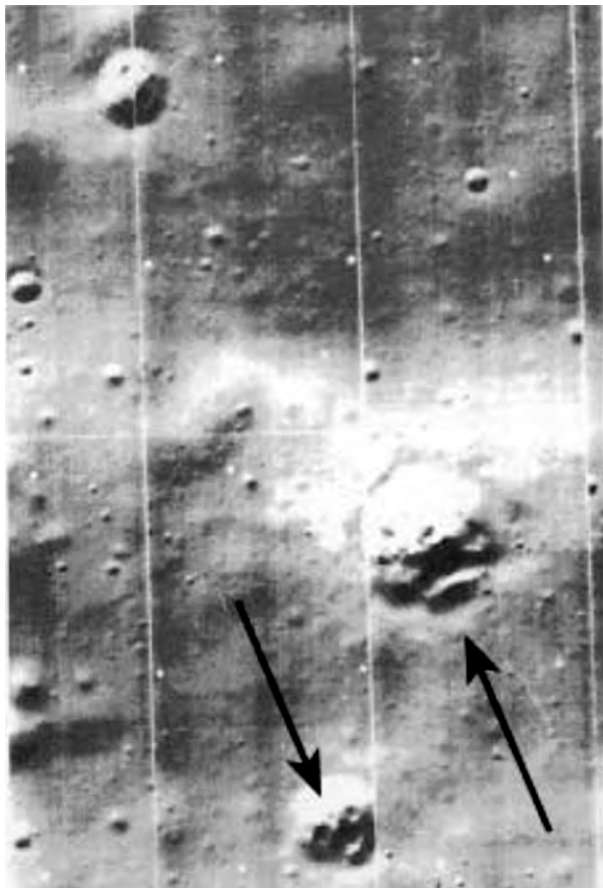
Fig. 127. Photo of LO 111, N194H3 (enlargement). It shows at least three craters with a type of construction inside.
