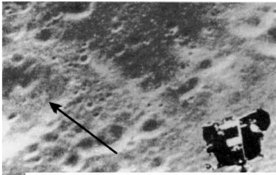
Fig. 83. LO III, M Photo: 67-H-201 (magnification). A large lofty Latin cross ('X') in the vicinity of the crater Kepler.
