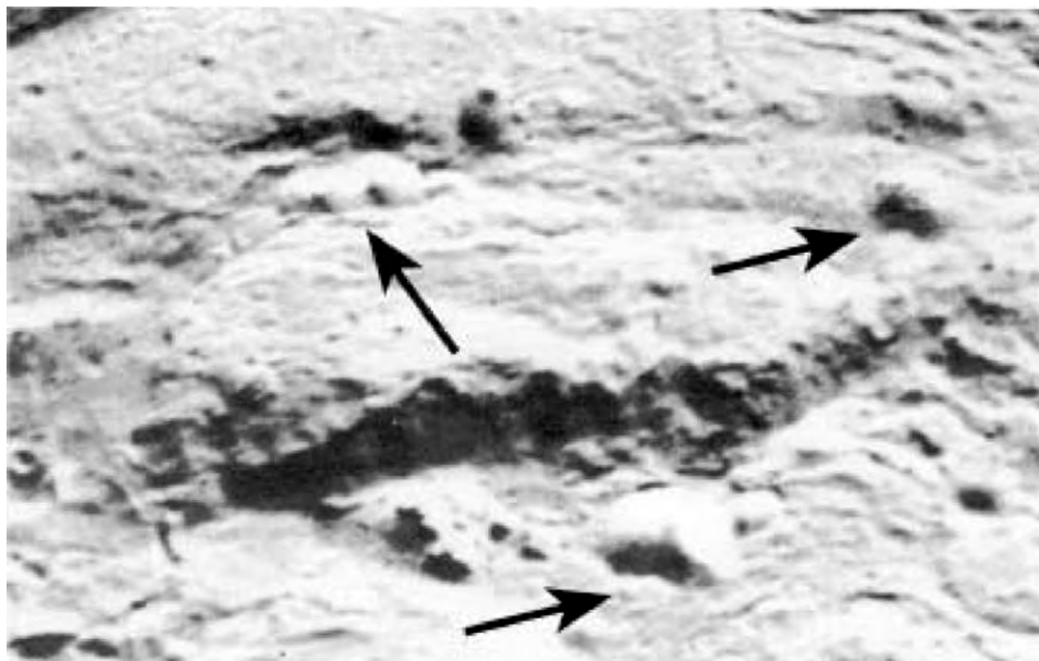
Fig. 36. Apollo 16, 16-19229 Ne Photo (enlargement). "The Domes" as they call NASA. Area around the crater King. The large dome in the center seems to be a double dome. (Moon back).
