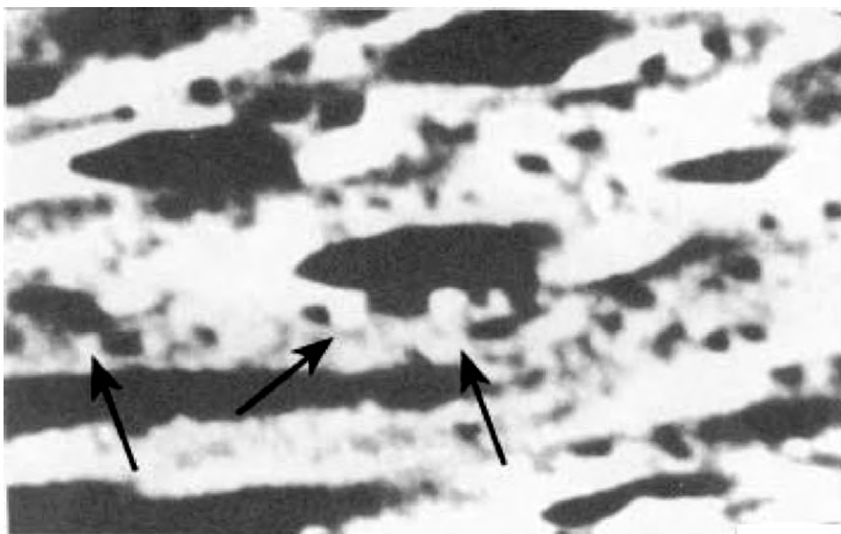
Fig. 133. On the 14x enlarged photo of Apollo 16, the towers or whatever they are also seen clearly.
