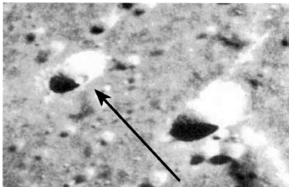
Fig. 35. Apollo 14, 14-10116 Ne Photo (Ausser i nittvergrerung). Even a cupola.
