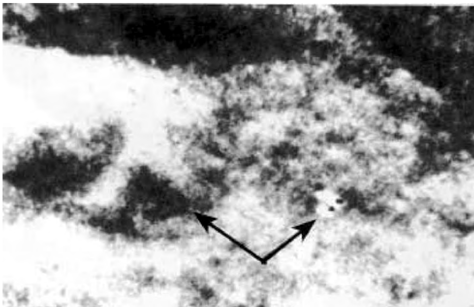
Fig. 131. (enlargement). The same three-sided pyramid-shaped constructs increased 14-fold. Note the two dark objects that are parked in the arrowhead-shaped clearing.
