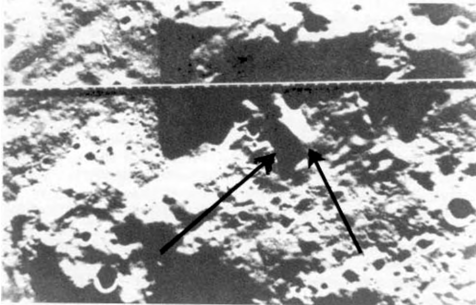
Fig. 5. Figure 6: Large platform south of the crater Archimedes. Discovered by Mr. Darling. Size of platform: 8 kilometers long and 1.6 kilometers wide, height: 1524 meters above the ground.
