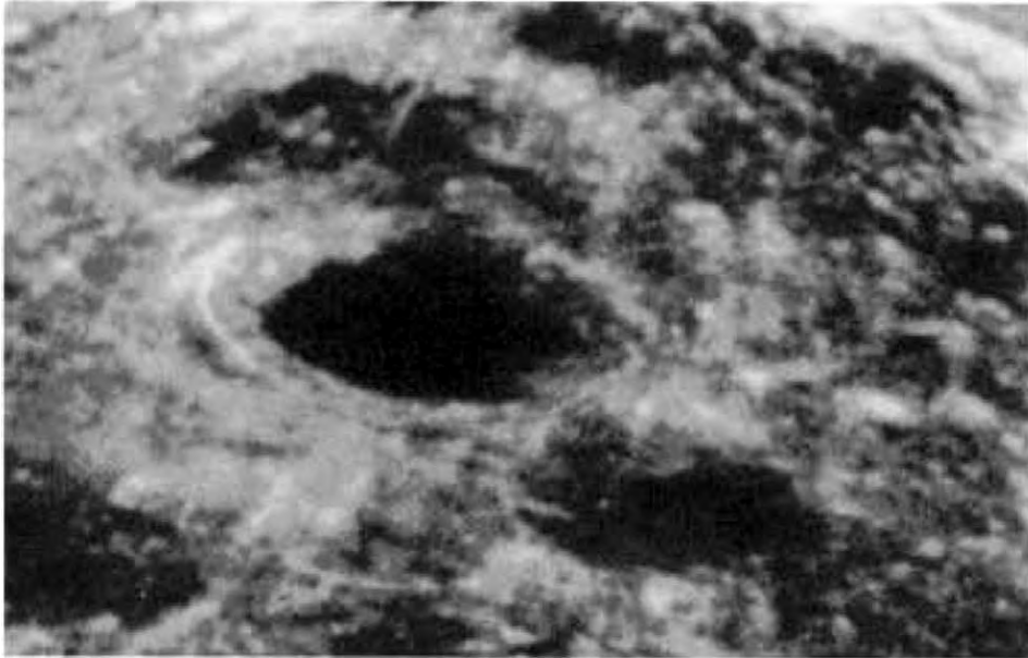
Fig. 53. Figure 47a: The lake. Note the objects on its banks
