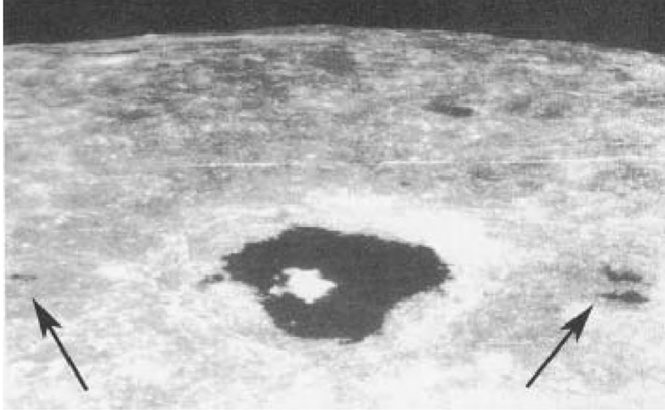
Fig. 50. NASA's Apollo 8 photo of the crater Tsiolkowski on the back of the moon. Note Be the large and small "lakes".
