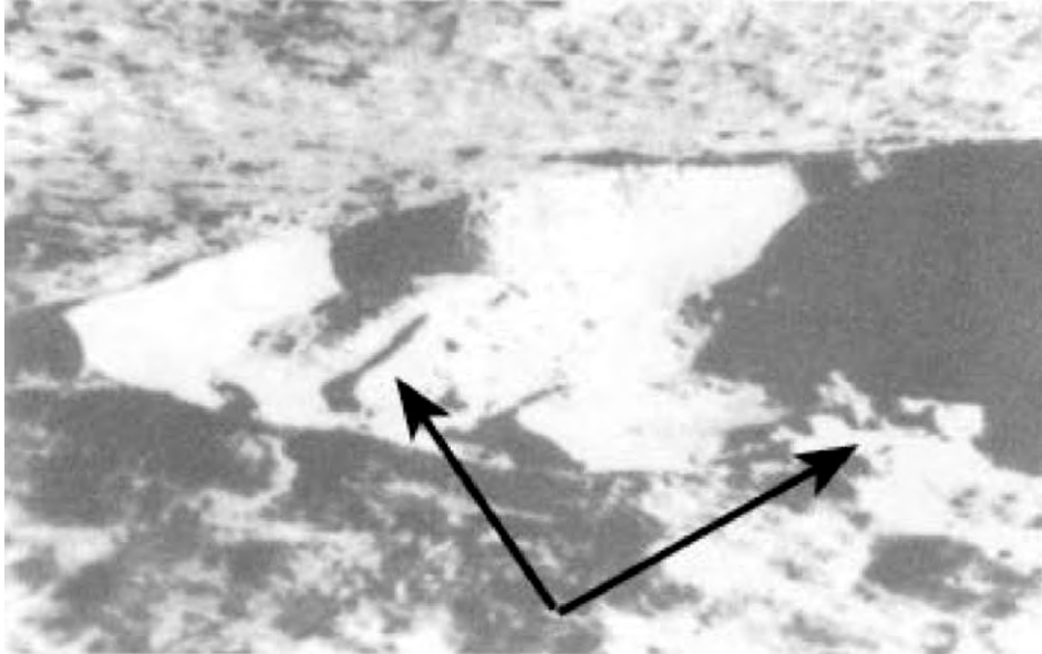
Fig. 31. NASA Luna. Orbiter 111, Photo No. 67-1-1-201 (enlargement). Close-up of the crater Kepler in Oceanus Procellarum. Notice the three domes on the crater rim to the right photo. Pay attention to the left ridge of the crater, which appears to have been cut or edited. Kepler has 32 kilometers in diameter:
