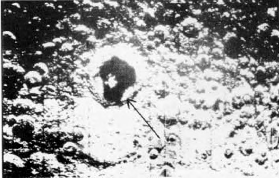
Fig. 51. Figure 46a: The crater Tsiolkowski, taken by Lunar Orbiter V NSAS.
