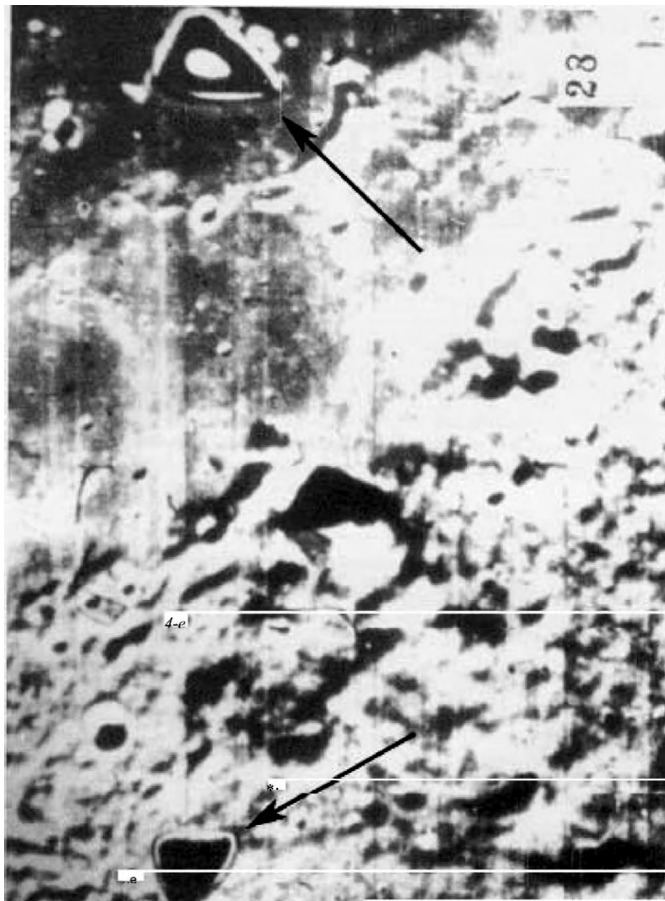
Fig. 54. NASA Luna / Orbiter IV photo No. HR 128 (enlargement), recorded in the vicinity of the crater Plato. Please refer to the two ponds or lakes above and below the picture that look like irrigation ponds. Also look out for the almond-shaped island in the upper lake.
