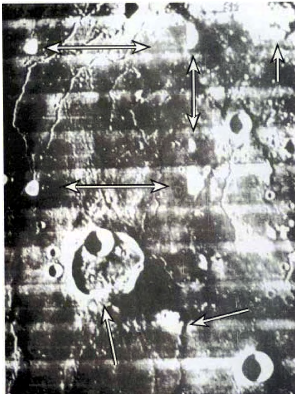
Fig. 58. Photo by NASA Lunar Orbiter IV, 151 'from the crater and its surroundings warriors. Note above five triangular white warriors, pond-like structures that reflect the sunlight-. Also look for the clouds at the edge of war as even fifty miles below the crater.
