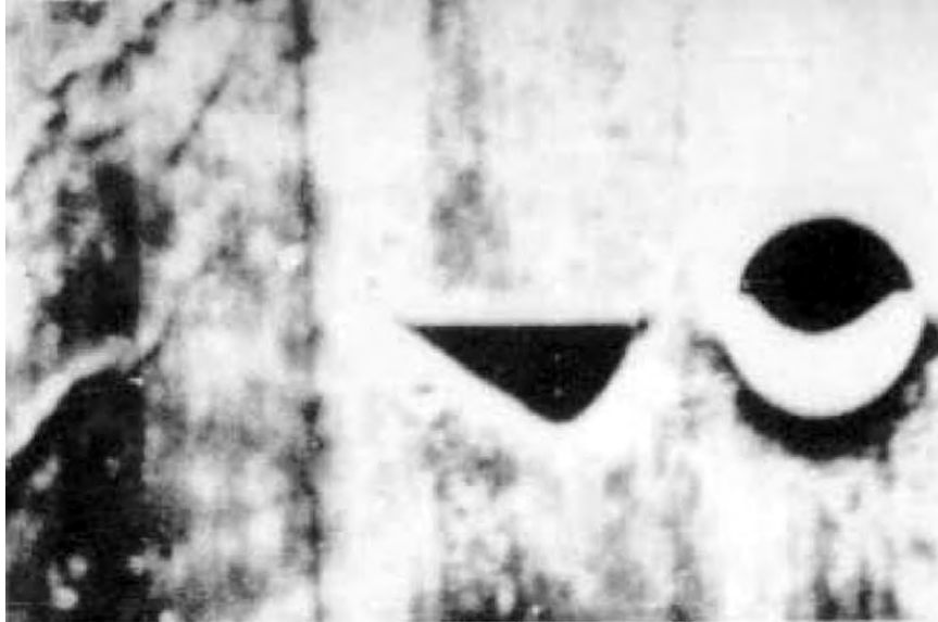
Fig. 61. Photo of Lunar Orbiter IV, No. 157 (enlargement), east of the crater Aristarchus. Two artificial-looking institutions: the perfectly formed crater and the 40-kilometer mountain or hangar.
