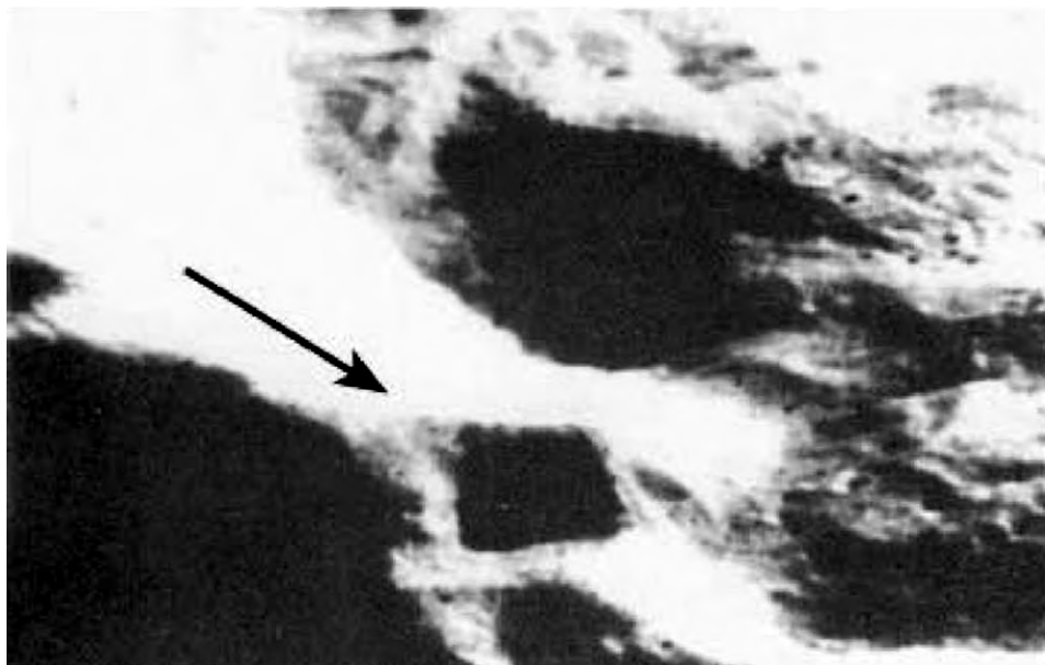
Fig. 126. This photo of Apollo 16 (enlargement) shows a square crater produced on the nature of the moon "square crater"?
