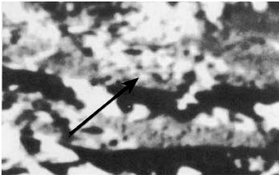
Fig. 112. Photo of Apollo, No. 10-324810 (enlargement), 209 kilometers north of the crater Triesnecker. Note the white bridge-like structure between two mountains
