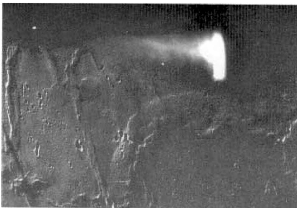
Fig. 100. Apollo 11 a glowing cigarette-shaped object near the moon in the
