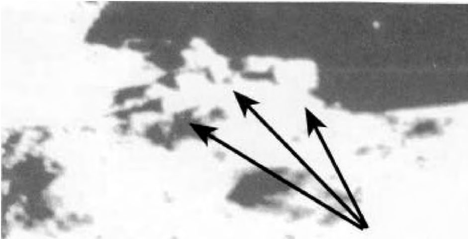
Fig. 32. NASA Luna / 'Orbiter III, Ne 67-H-201 (enlargement). The three domes in the center of the crater Kepler closely. You are really on a large platform at the edge of the crater.
