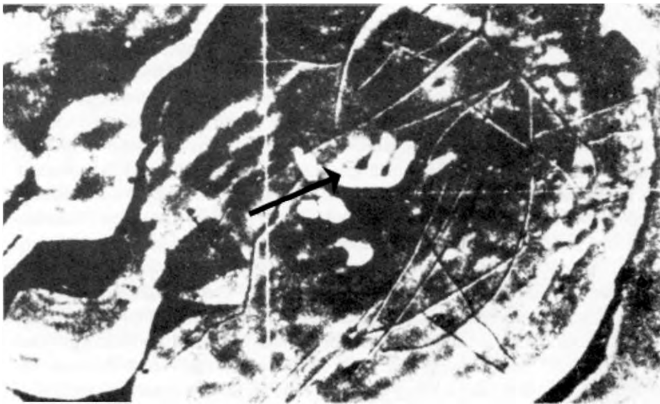
Fig. 3. Figure 4: The Gassendi crater, taken 45 years ago with the 100-inch telescope (2.54 meters) at Mount Wilson Observatory. Note the tube system in the Gassendi-sole. Note also the mountain in the middle, which was cut to a platform that represents the letter "e".
