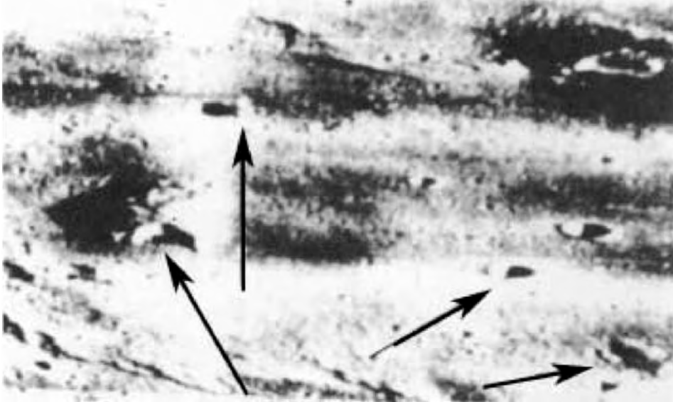
Fig. 55. Photo by NASA Lunar Orbiter 11, No. MR 213 (enlarged). Note that the hill on the left seems to be cut from the middle like a piece of a cake. Also look for the large radar dome-like over the hill, which casts a shadow to the left. Note the right of the picture perfect cut several holes (or crater?) And two oval objects.
