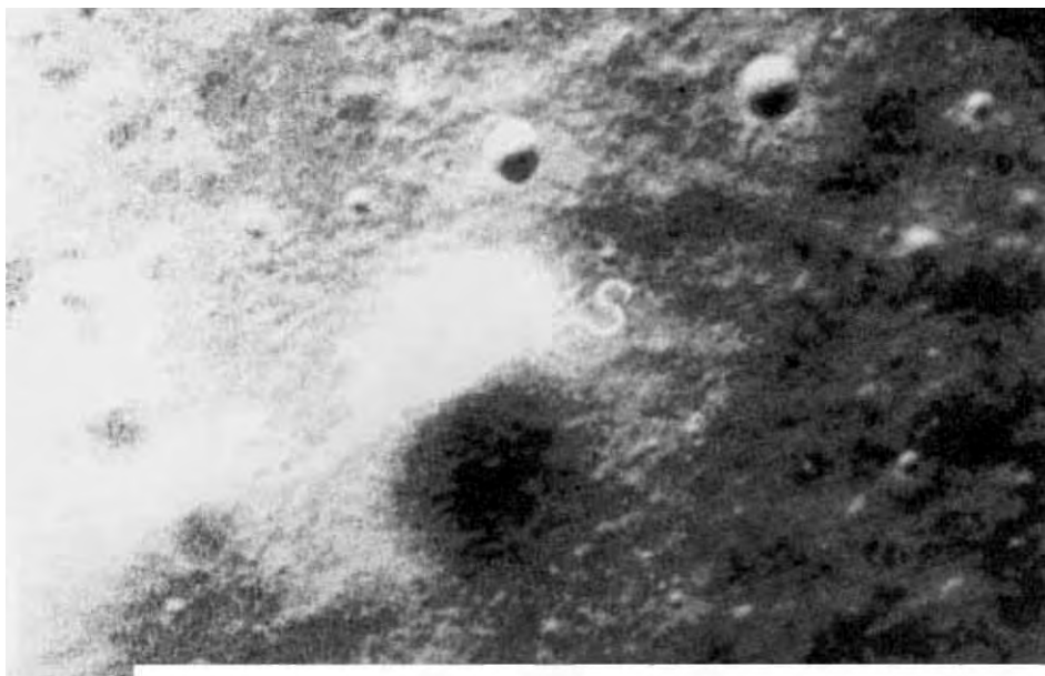
Fig. 110. Photo of Apollo 14, Ne 14-80-10439. Another letter "S". This time, besides this crater.
