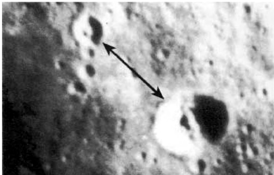
Fig. 123. Photo by Lunar Orbiter III, No. 6H. It shows smoke rising from the bottom of a crater. Note also the white dome in the crater to the northwest.
