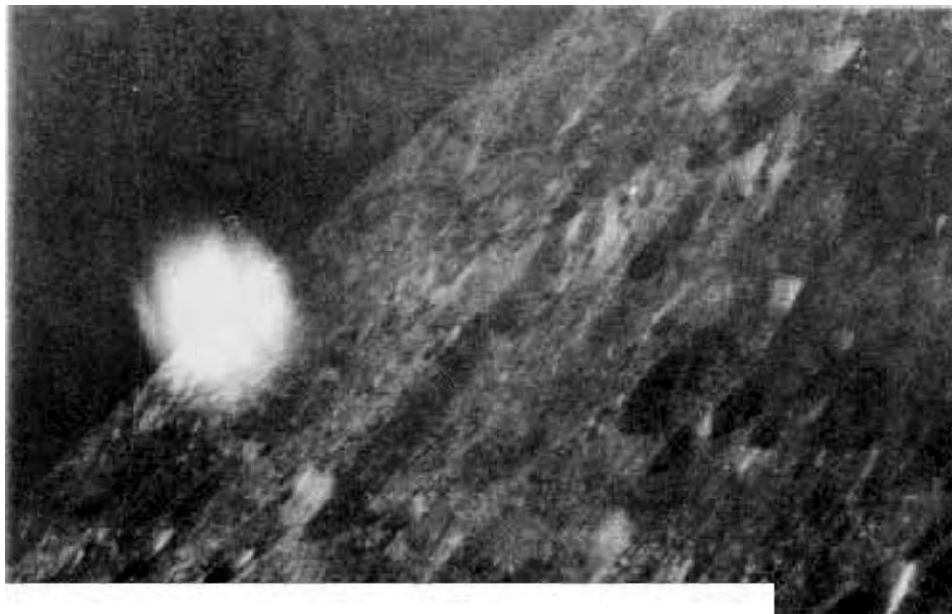
Fig. 93. Figure 87: NASA AS No. 13-60-8609. Apollo 13 photo of a UFO. on the Moon
