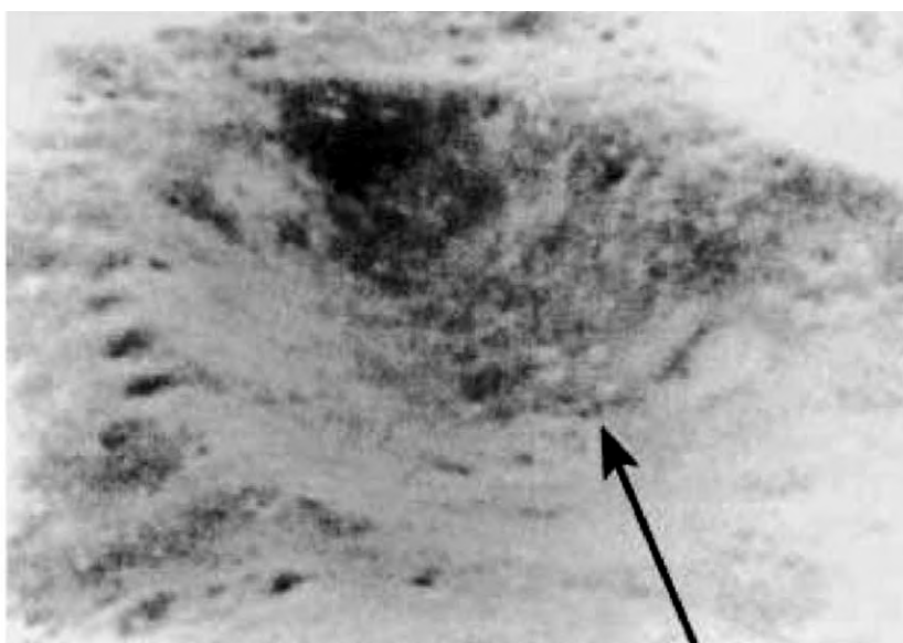
Fig. 106. Figure 100: Photograph of Apollo 10, Ne unknown. Four white egg-shaped objects in the large craters are parked.
