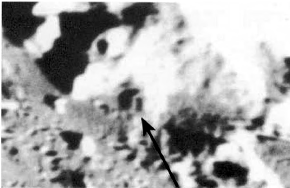
Fig. 111. Photo of Apollo 10, No. 10-32-4810 (enlargement), 130 kilometers north of Triesnecker Note the cathedral-like entrance, which was cut into the mountain
