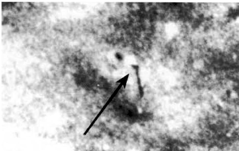
Fig. 118. Photo of Apollo 16, Ne 19 386 (enlargement). Please note a kind of tube or pipe that looks like a spiral. It leads from the bottom to the smaller crater about it. Note the seven or more rings around this strange object.
