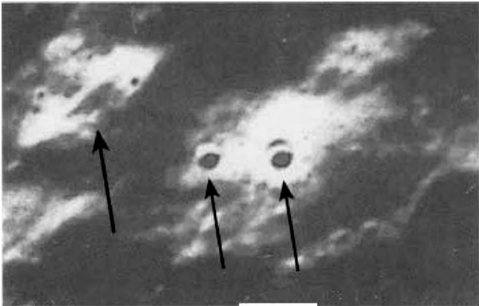
Fig. 135. Figure 129: NASA photo Ne 67 H 1651st Middle: Apparently concentric Dome structures. Top left: Apparently a bridge-like structure. Note the shadow underneath
