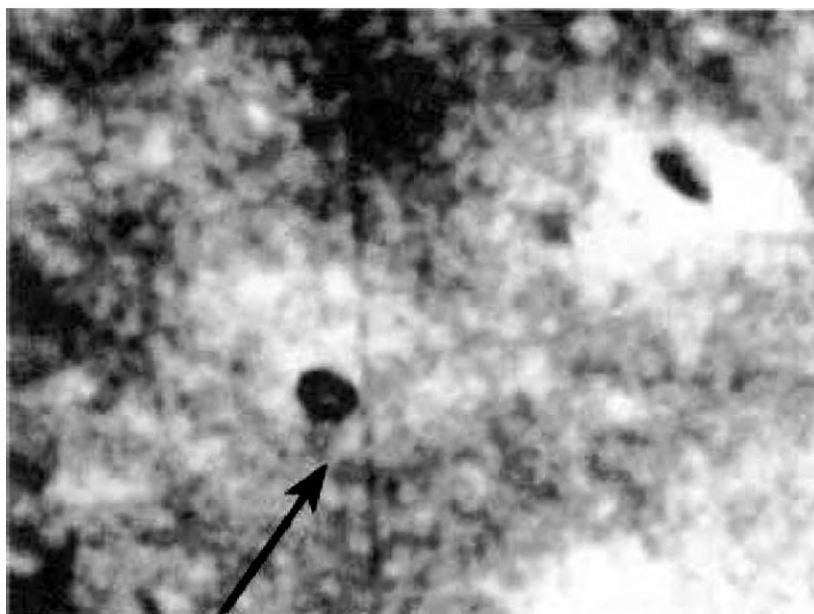
Fig. 122. Apollo 16, No. 16-19386 (enlargement). This photo shows a small pond with an island at the bottom of a shallow crater. Note the long spiraling tube that runs from north to south next to the edge of the crater. They turn the principle of the Archimedean screw?
