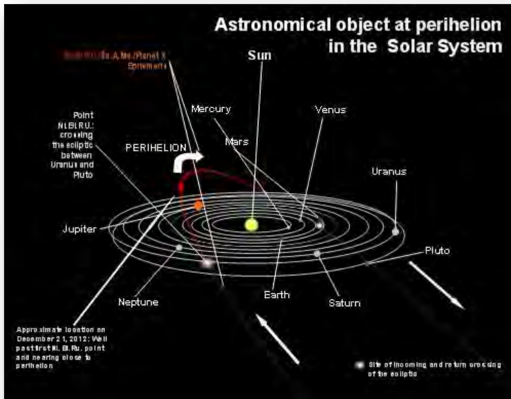
Figure 1-4A. The red line indicates Ša.AM.e's supposed orbit when it enters and leaves our solar system. The red planet on the line is Ša.AM.e/Nibiru's estimated position on December 21, 2012, according to LPG-C.
