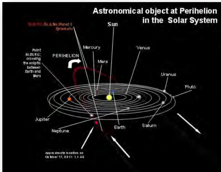
Figure 1-4. The red line indicates Ša.AM.e's supposed orbit when it enters and leaves our solar system. The red planet on the line is Ša.AM.e/Nibiru's position on October 17, 2011, then approx. 1AU from Earth -- more exactly 93,000,000 miles + an extra 17,000-18.000 miles more, according to LPG-C. (Better resolution below)
