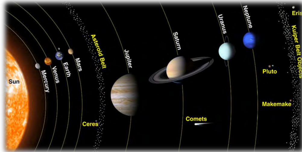
Figure 1-1. Model of our solar system. In ancient times, Earth was located between Mars and Jupiter, where today's asteroid belt is.
