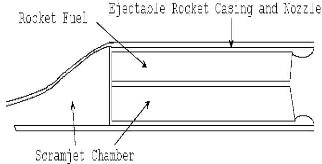
Figure 3-3. Rocket/Dump Combustor Scramjet.
