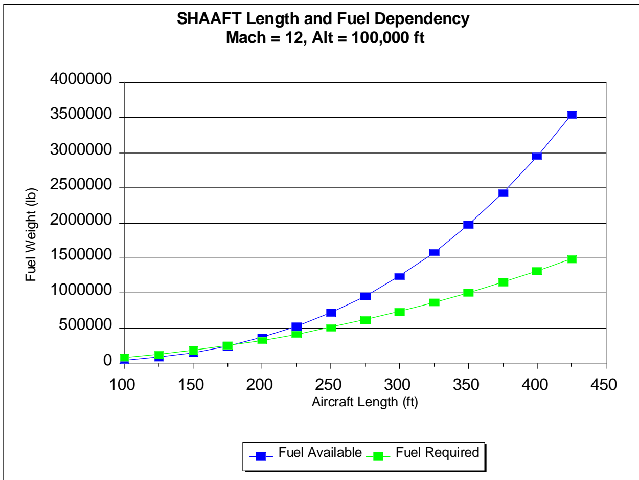
Figure 2-6. SHAAFT Sizing.
