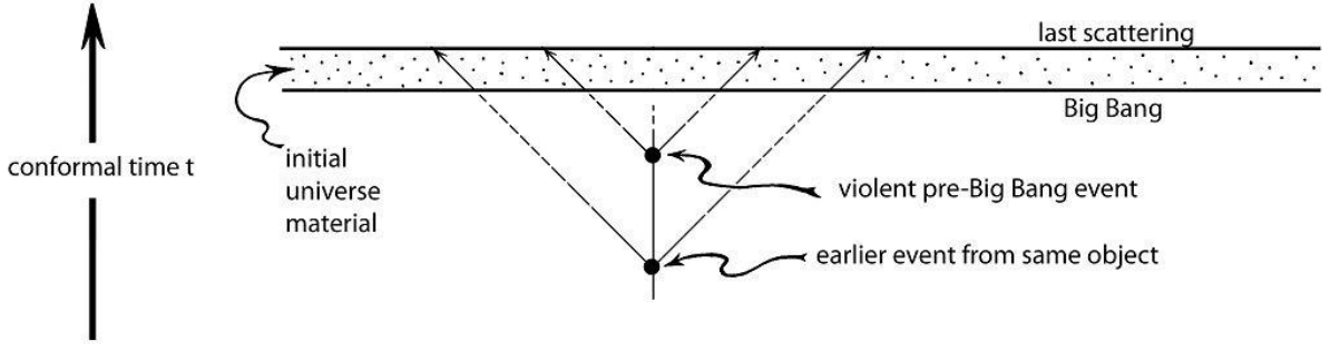
Figure 1. Conformal diagram (without inflation) of the effect, according to CCC, of a pre-Big-Bang entity (a supermassive black-hole encounter, according to CCC which is the source of two violent events).
