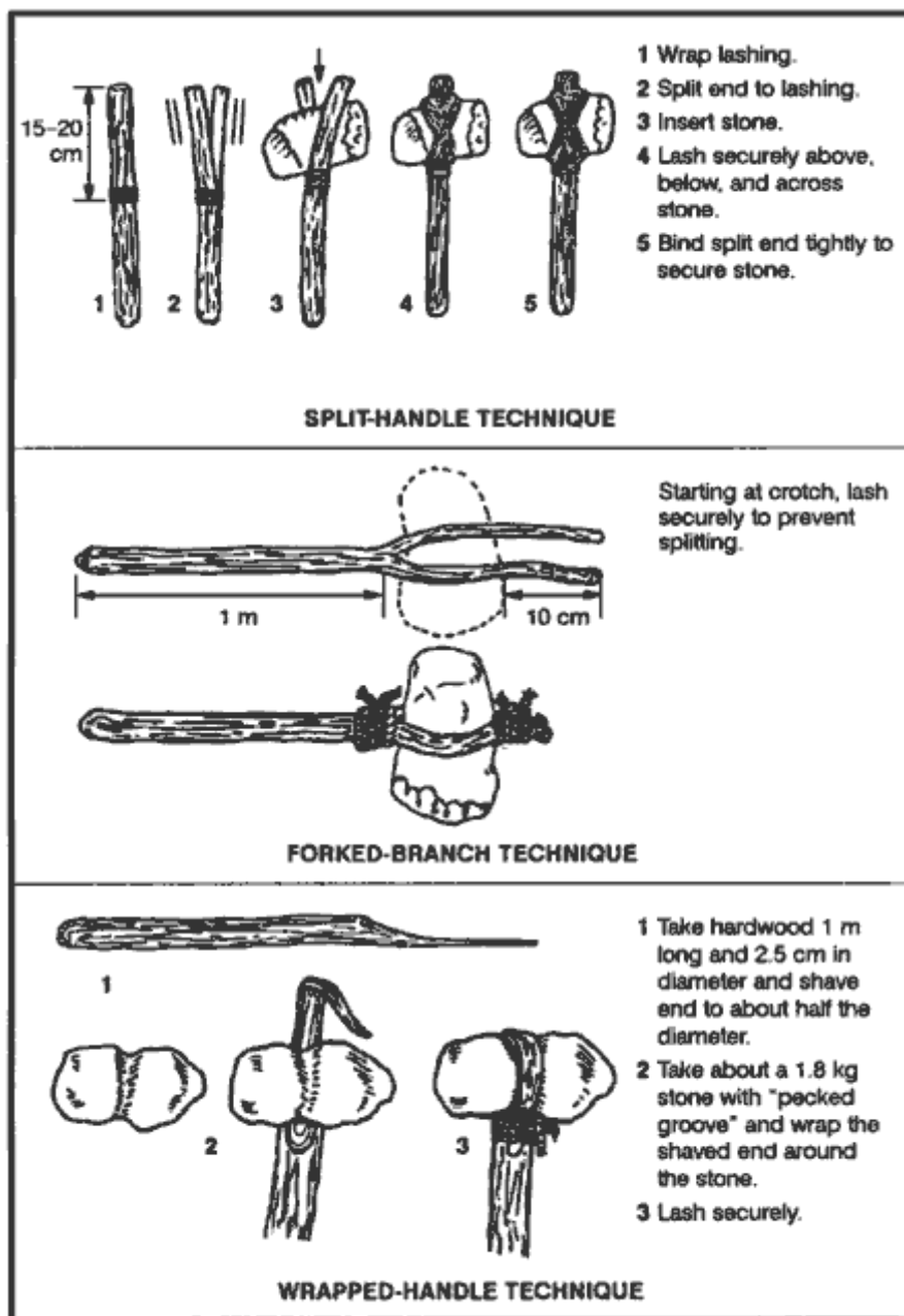
Figure 12-1. Lashing clubs.
