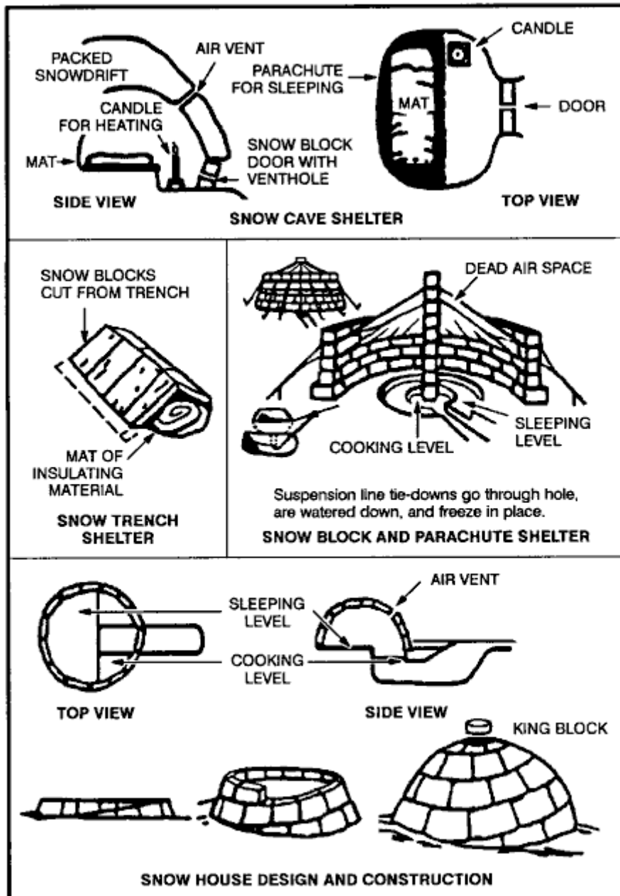
Figure 15-4. Snow houses.
