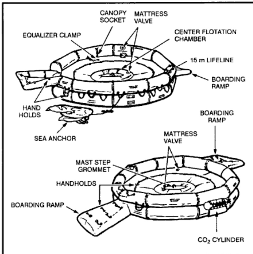
Figure 16-15. Twenty-man raft.
