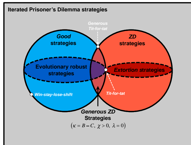
Fig. 2. Relationship between ZD and good strategies in the IPD. The intersection between ZD and good is precisely the set of generous ZD strategies. Not all good strategies are generous. As a result, only a strict subset of good strategies is evolutionary robust, just as a strict subset of ZD strategies is evolutionary robust. Extortion strategies are neither generous nor evolutionary robust. Also shown are the locations of the classic IPD strategies (19) win-stay-lose-shift, tit-for-tat, and generous tit-for-tat.
