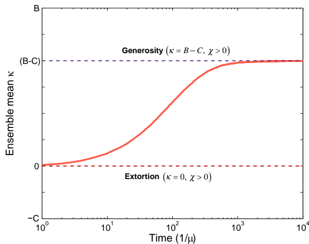
Fig. 1. Evolution from extortion to generosity within the space of ZD strategies. Populations were simulated in the regime of weak mutation. The figure shows the ensemble mean value of \kappa in the population, plotted over time. The expression \kappa=0 corresponds to the extortion strategies of Press and Dyson (1), whereas \kappa=B-C corresponds to the generous ZD strategies. Each population was initialized at an extortion strategy E_\chi , with \chi drawn uniformly from the range \chi \in (0,1) . Given a resident strategy in the population, mutations to \kappa were proposed as normal deviates of the resident strategy, truncated to constrain \kappa \in [0, B-C] , whereas mutations to \{\chi, \phi\} were drawn uniformly from \max\left(\frac{\kappa-B}{\kappa+C}, \frac{\kappa+C}{\kappa-B}\right) \leq \chi \leq 1 with \phi drawn uniformly within the feasible range, given \kappa and \chi . A proposed mutant strategy replaces the resident strategy with a fixation probability dependent on their respective payoffs, as in the work of Hilbe et al. (12) and Traulsen et al. (20). The mean \kappa among 10^3 replicate populations is plotted as a function of time. Parameters are B=3 , C=1 , N=100 , and selection strength \sigma=1 .
