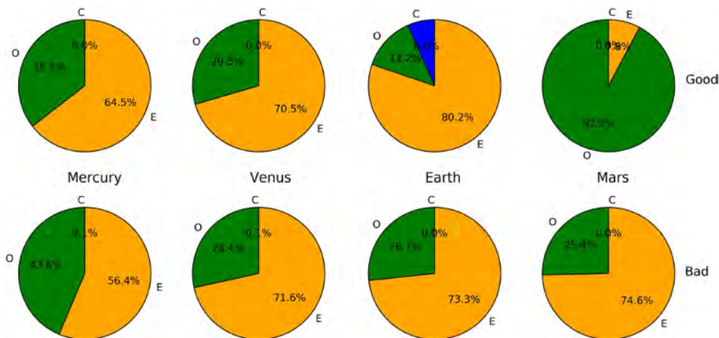
Fig. 5. Pie chart of the composition of the terrestrial planets for the successful simulation, corresponding to Fig. 3 (top), and the unsuccessful simulation in Fig. 4 (bottom). Labels indicate which chart corresponds to what planet analogue. Enstatite chondrite is in orange, ordinary chondrite in green and carbonaceous in blue. In the top case the Earth analogue accreted some carbonaceous chondrite material. Note that the successful case has a composition for Mars that is strikingly different than that of the other three planets. (For interpretation of the references to colour in this figure legend, the reader is referred to the web version of this article.)
