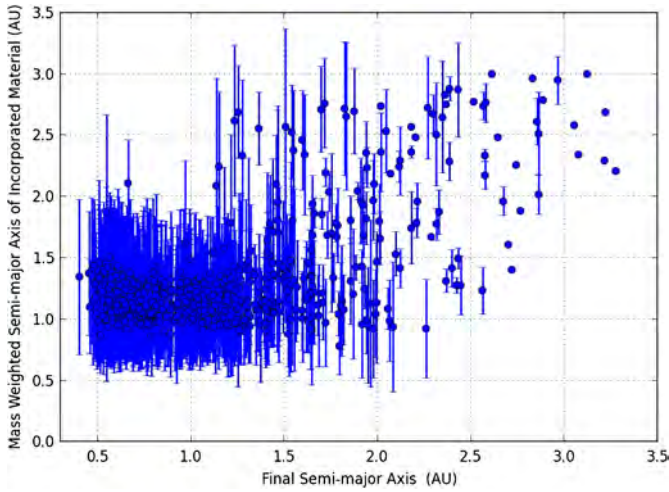
Fig. 2. Mass-weighted initial semi-major axis of material incorporated into the planets as a function of their final semi-major axis. The Grand Tack clears the disc beyond 1 AU and mixes in some material from farther out, so that there are many planets that only sample the inner disc.
