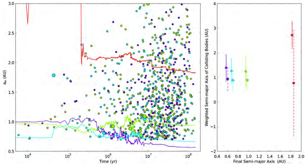
Fig. 3. Dynamical evolution of an extreme case that yields a Mars analogue that is compositionally different from the Earth and Venus because it samples a distinctly different region of the protoplanetary disc. The left panel indicates the evolution of the semi-major axis of the four terrestrial planet analogues and the coloured dots indicate the initial semi-major axis and time of bodies that collide with the terrestrial planet analogues. The size of the dots is indicative of their mass. The Mars analogue gets scattered first outwards and then inwards by Jupiter and slowly migrates towards 1.8 AU through dynamical interaction with the remaining planetesimals. The right panel indicates the mass-weighted mean initial semi-major axis of material that is incorporated into the four terrestrial planet analogues. The error bars depict the total range of material incorporated into the final planets in the Grand Tack model while the dotted error bars are the same if we suppose the planets originated from the same narrow region between 0.7 AU and 1 AU as in the annulus model. (For interpretation of the references to colour in this figure legend, the reader is referred to the web version of this article.)
