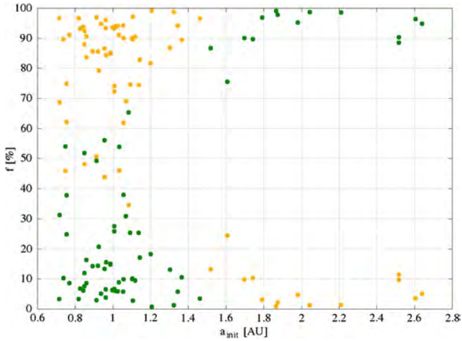
Fig. 6. Scatter plot of the percentage of enstatite (orange) and ordinary chondrite (green) compositional make-up of all Mars analogues. Two dots are plotted for each planet, with the combined values adding up to 100%. (For interpretation of the references to colour in this figure legend, the reader is referred to the web version of this article.)
