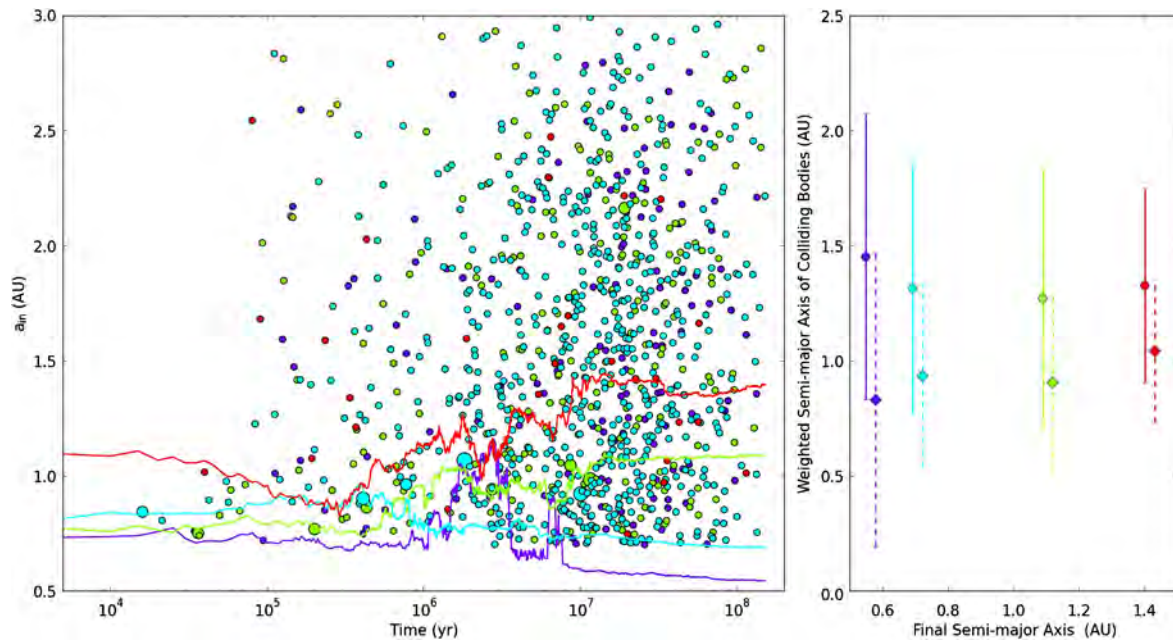
Fig. 4. Same as Fig. 3 but now we show a case where the composition of the Mars analogue is nearly identical to that of the Earth analogue because they sample the same region of the protoplanetary disc. (For interpretation of the references to colour in this figure legend, the reader is referred to the web version of this article.)
