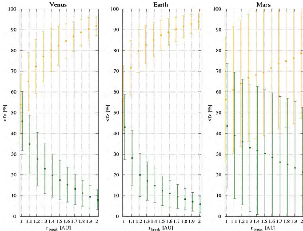
Fig. 7. Scatter plot of the average percentage contribution of enstatite (orange) and ordinary chondrite (green) to the bulk compositions of Venus, Earth and Mars. Data are plotted as a function of the distance where the disc changes its composition from one meteorite class to another. (For interpretation of the references to colour in this figure legend, the reader is referred to the web version of this article.)
