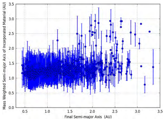
Fig. 8. Mass-weighted initial semi-major axis of material incorporated into the planets as a function of their final semi-major axis for the set of Grand Tack simulations with the tack at 2 AU. Note that the majority of planets still only sample the inner part of the disc and that this region now extends to beyond 2 AU.
