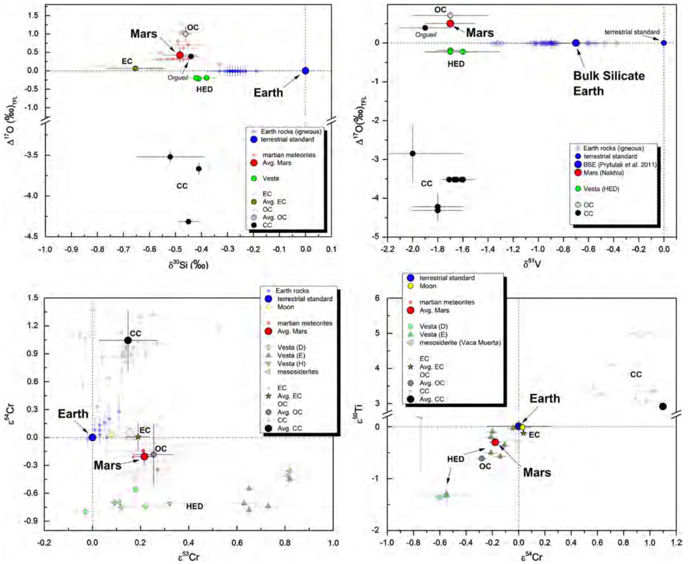
Fig. 1. Four-panel plot of the correlated comparative isotopic compositions of Earth (and Moon), Mars, Vesta (howardites, eucrites, diogenites, mesosiderites), EC (enstatite chondrites), OC (ordinary chondrites), and CC (carbonaceous chondrites). All data are normalised according to the terrestrial standard values. We only plot correlated data by sample, and not just averages, for each meteorite group. As such, differences that exist between different samples in, for example oxygen isotopes in the HEDs, become highlighted. Top-left: correlated oxygen vs. silicon. Top-right: correlated oxygen vs. vanadium. Bottom-left: correlated multiple chromium isotopes ( ^{53}\text{Cr} and ^{54}\text{Cr} ). Bottom-right: correlated titanium and chromium isotopes ( ^{50}\text{Ti} and ^{54}\text{Cr} ).
