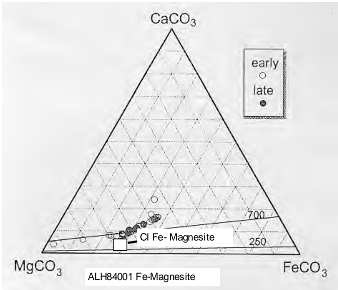
Figure 10. A comparison of the composition of ferrous magnesite found in ALH84001 and that found its CIs (adapted from Wright I.P., M.M. Grady, and C.T. Pillinger. 1992).
