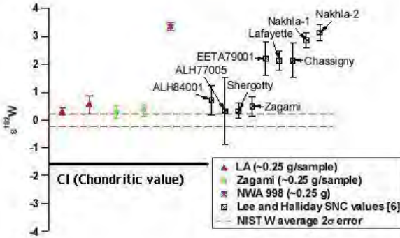
Figure 6. A comparison of Mars and Terrestrial Tungsten isotopes with those of CI.
