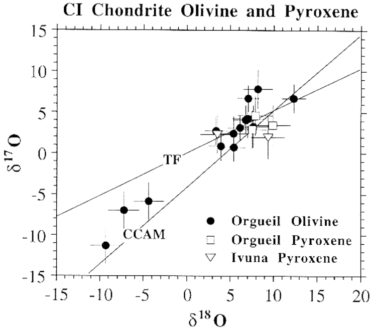
Figure 3. A graph of oxygen isotopes for CI olivine and pyroxene grains compared to a representative MM olivine form from the MM Chassigny.
