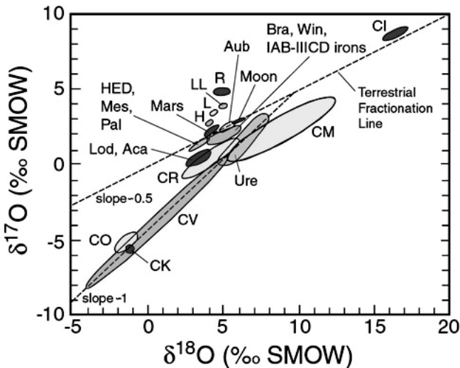
Oxygen isotopes of meteorites (JPL/NASA)
