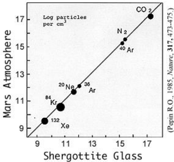
A graph of Mars atmosphere versus trapped gases in Mars meteorites
