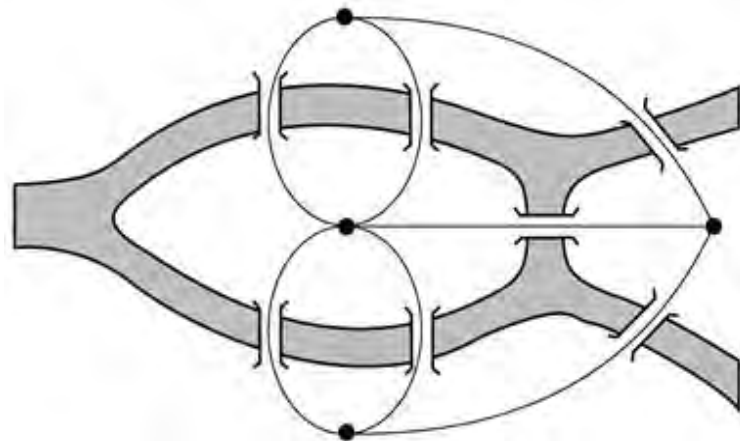
Figure 2. Diagram of the Bridges of Königsberg
