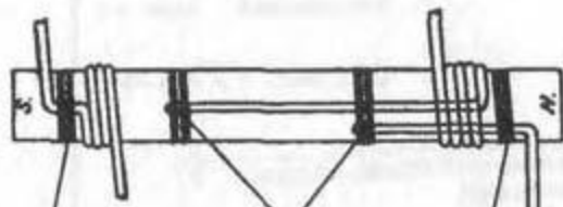
binding soldered & bound binding Note: Paper insulation between magnet and coil. Rys.1
