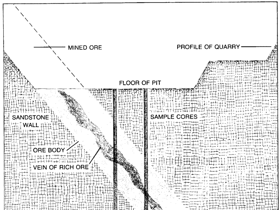
ORE BODY AT OKLO , shown in a schematic profile of the mine, lies above a sandstone wall with an average slope of about 45 degrees. The reactor zones are within the rich vein of ore, which is roughly a meter thick. The zones generally have a lenticular cross section. The extent of the ore body and the location of the reactor zones were revealed by removing core samples.
