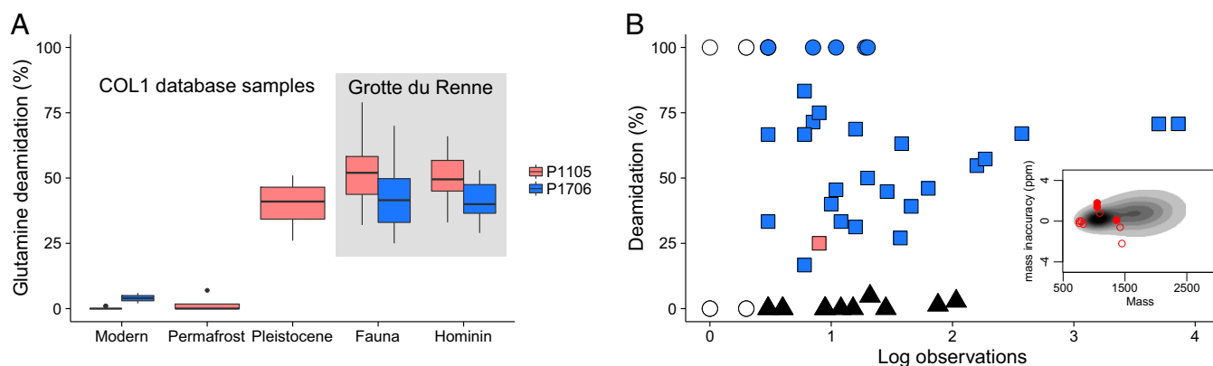
Fig. 1. Identification of damaged ancient proteins. ( A ) Deamidation values of bone ammonium-bicarbonate extracts for database samples and Arcy bone specimens analyzed using MALDI-TOF-MS. ( B ) Deamidation frequency based on spectral counts obtained through LC-MS/MS analysis. Cluster analysis provides three clusters (filled triangles, squares, and circles). Open circles represent proteins that have two or fewer spectral matches and were not included in cluster analysis. COL1 \alpha 1 is indicated in pink; 0% indicates no deamidation and 100% indicates complete deamidation. ( Inset ) AR30 ppm error distribution by peptide mass for assigned spectra, with spectra matching to COL1 \alpha 1 in red, open circles and those to COL1 \alpha 1 128N in red, filled circles.
