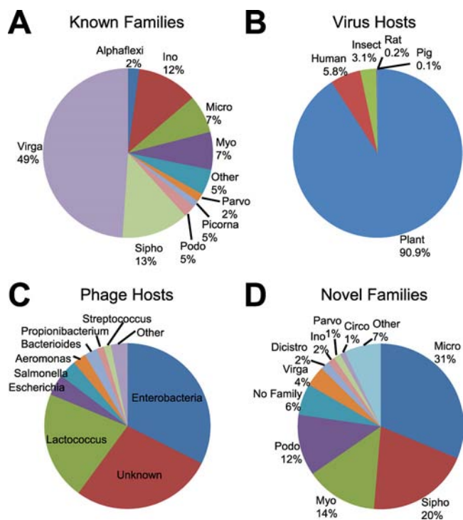
FIG 2 Raw sewage contains many known and novel viruses. (A) Known viral sequences ( n = 3,027 ) identified by BLAST are related to many different viral families. Families with <1\% abundance were collapsed into the “Other” category. Only the prefixes of family names are shown (e.g., Virga for Virgaviridae ). (B) Distribution of the hosts of the known eukaryotic virus reads ( n = 1,748 ). Plant, human, and insect viruses are abundant in raw sewage. (C) Distribution of the hosts of the known bacteriophage reads ( n = 1,279 ). (D) Novel sequences ( n = 43,381 ) identified by BLAST are related to many different virus families. Families with <1\% abundance were collapsed into the “Other” category. See Table S6 for a list of families and hosts in the “other” category.
