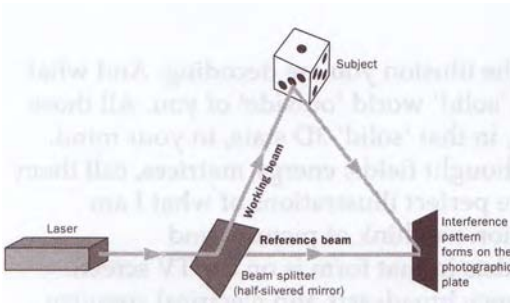
Figure 14: How a hologram is made. One part of the laser light (the 'working beam') is deflected onto the subject and then onto a photographic plate. The other part (the 'reference beam') is directed straight at the photographic plate. When the two parts collide they form an interference pattern that is a waveform version of the subject being photographed
