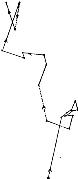
Tropæolum majus : heliotropic movement and circumnutation of an old internode towards a lateral light, traced on a horizontal glass from 8 A.M. Nov. 2nd to 10.20 A.M. Nov. 4th. Broken lines show the nocturnal course.
