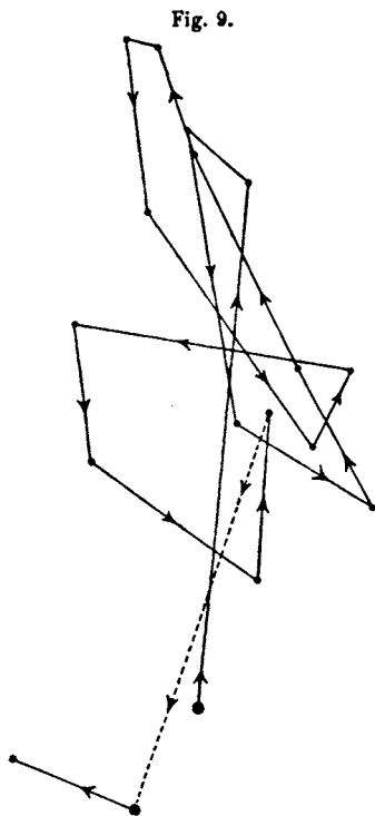
Fig. 9. Brassica oleracea : circumnutations of hypocotyl, in darkness, traced on a horizontal glass, by means of a filament with a bead fixed across its summit, between 9.15 A.M. and 8.30 A.M. on the following morning. Figure here reduced to one-half of original scale.
