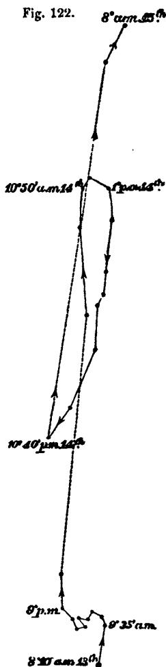
Ampelopsis tricuspidata : hypnastic movement of hooked tip of leading shoot, traced from 8.10 A.M. July 13th to 8 A.M. 15th. Apex of shoot 5\frac{1}{2} inches from the vertical glass. Plant illuminated through a skylight. Temp. 17\frac{1}{2}^{\circ} – 19^{\circ} C. Diagram reduced to one-third of original scale.
