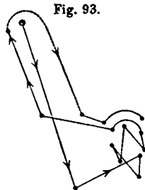
Sarracenia purpurea : circumnutation of young pitcher, traced from 8 A.M. July 3rd to 10.15 A.M. 4th. Temp. 17°-18° C. Apex of pitcher 20 inches from glass, so movement greatly magnified.
