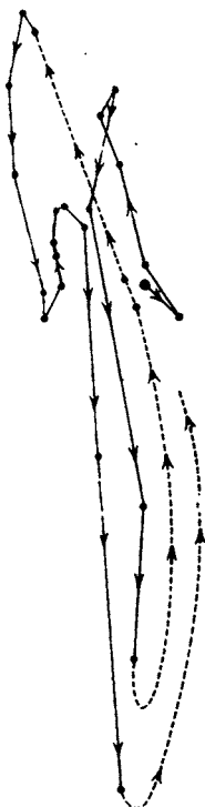
Portiera hygrometrica : circumnutation and nyctitropic movements of petiole of leaf, traced from 9.35 A.M. July 7th to about midnight on the 8th. Apex of leaf 7½ inches from the vertical glass. Temp. 19½°–20½° C.
