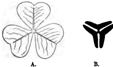
Oxalis aetosella : A, leaf seen from vertically above; B, diagram of leaf asleep, also seen from vertically above.
