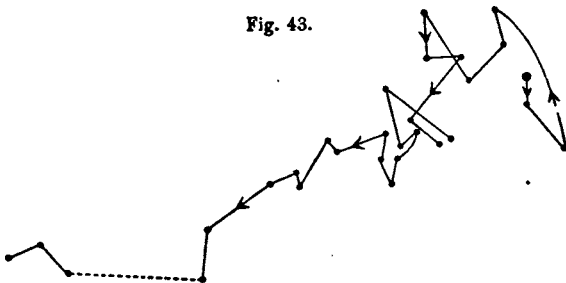
Pinus pinaster : circumnutation of hypocotyl, with filament fixed across its summit, traced on horizontal glass, from 10 A.M. March 21st to 9 A.M. 23rd. Seedling kept in darkness. Movement of bead magnified about 85 times.
