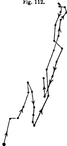
Acanthus mollis : circumnutation of young leaf, traced from 9.20 A.M. June 14th to 8.30 A.M. 16th. Apex of leaf 11 inches from the vertical glass, so movement considerably magnified. Figure here reduced to one-half of original scale. Temp. 15^{\circ} – 16\frac{1}{2}^{\circ} C.
