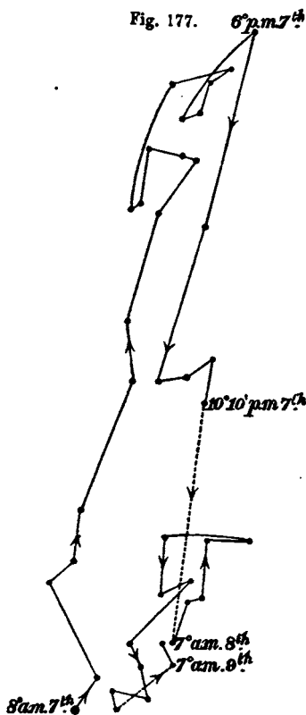
Cassia tora : heliotropic movement and circumnutation of a hypocotyl. ( 1\frac{1}{2} inch in height) traced on a horizontal glass from 8 A.M. to 10.10 P.M. Oct. 7th. Also its circumnutation in darkness from 7 A.M. Oct. 8th to 7.45 A.M. Oct. 9th.
