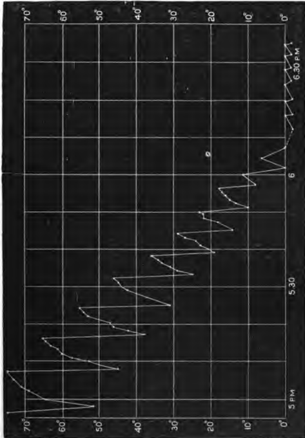
Aterrhoa bilimbi : angular movements of a leaflet during its evening descent, when going to sleep. Temp. 78°-81° F.
