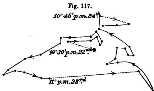
Crinum capense : circumnutation of dependent tip of young leaf, traced on a bell-glass, from 10.30 P.M. May 22nd to 10.15 A.M. 25th. Figure not greatly magnified.
