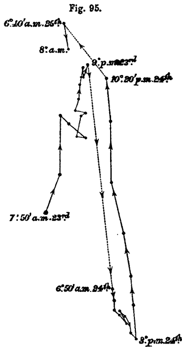
Cr. imbe maritima : circumnutation of leaf, disturbed by being insufficiently illuminated from above, traced from 7.50 A.M. June 23rd to 8 A.M. 25th. Apex of leaf 15¼ inches from the vertical glass, so that the tracing was much magnified, but is here reduced to one-fourth of original scale.
