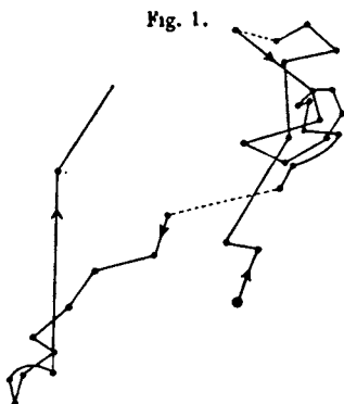
Brassica oleracea : circumnutating of radicle, traced on horizontal glass, from 9 A.M. Jan. 31st to 9 P.M. Feb. 2nd. Movement of bead at end of filament magnified about 40 times.
