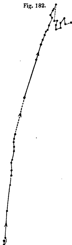
Cytisus fragrans : apogeotropic movement of stem from 10^\circ beneath to 60^\circ above horizon, traced on vertical glass, from 8.30 A.M. March 12th to 10.30 P.M. 13th. The subsequent circumnutating movement is likewise shown up to 6.45 A.M. on the 15th. Nocturnal course represented, as usual, by a broken line. Movement not greatly magnified, and tracing reduced to two-thirds of original scale.
